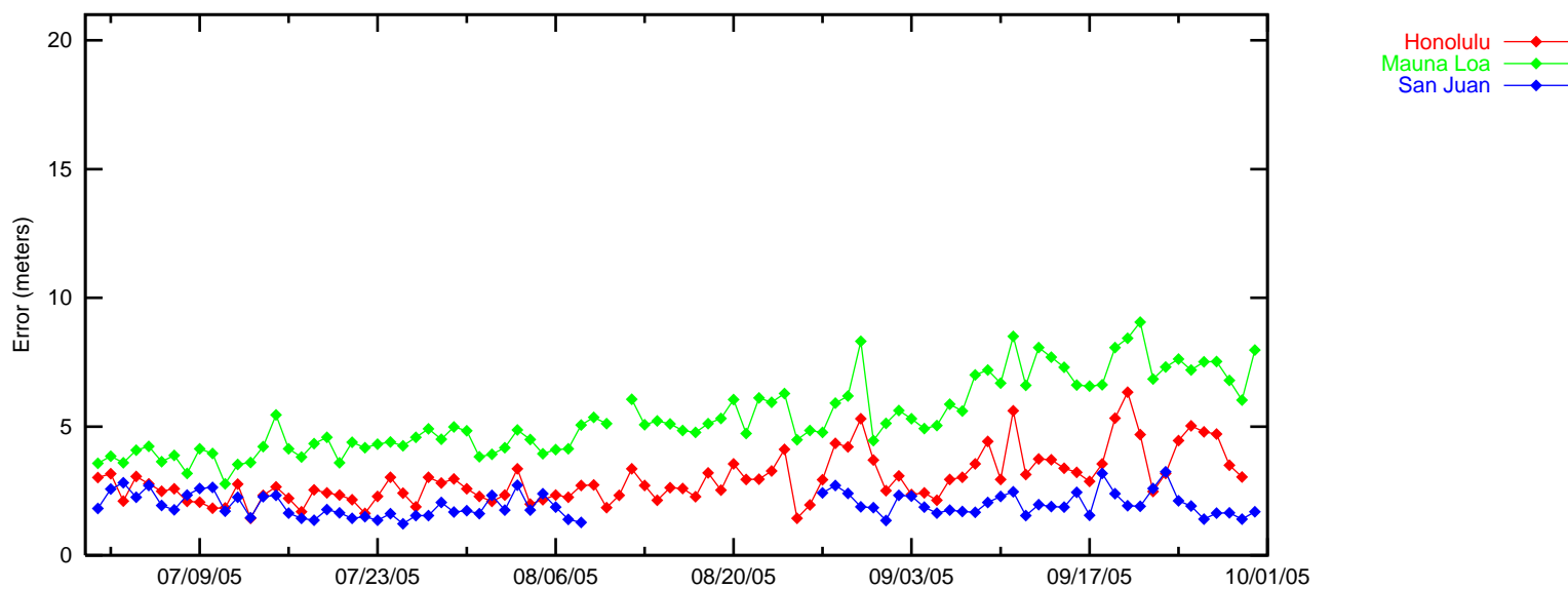
Figure 2-5 NPA 95% Horizontal Accuracy
