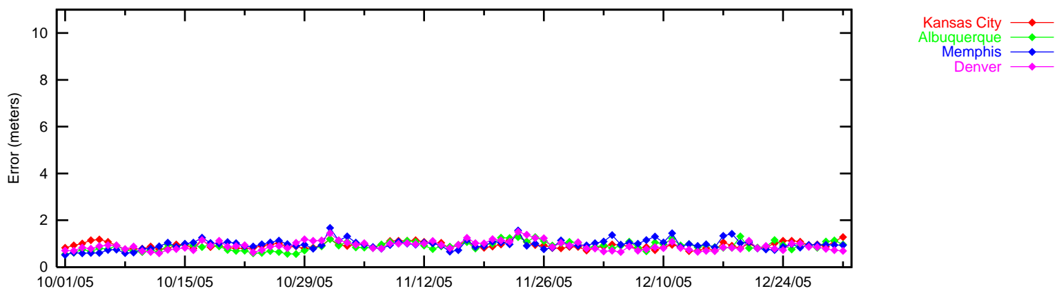
Figure 2-2 95% Horizontal Accuracy at LNAV/VNAV
