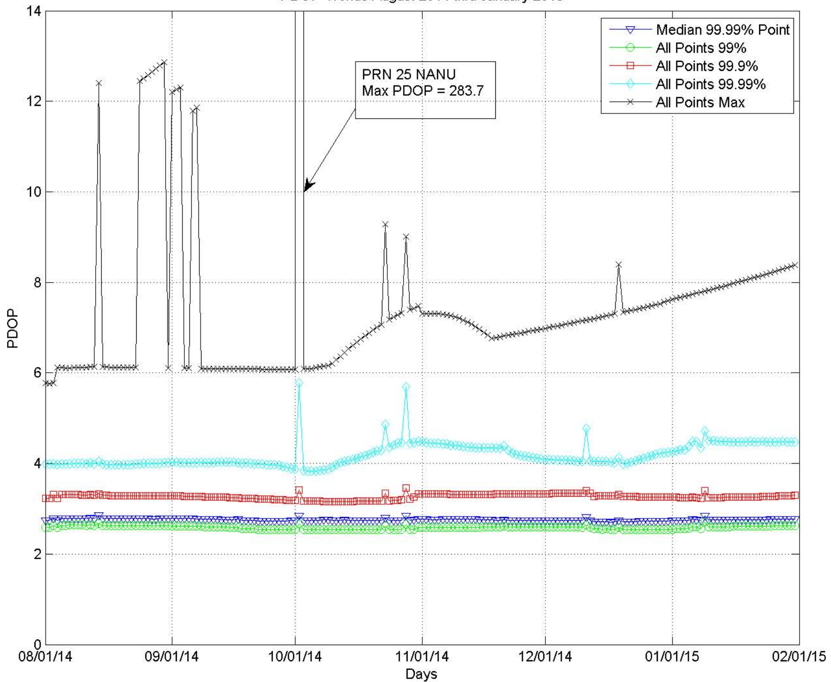
PDOP Trends August 2014 thru January 2015
