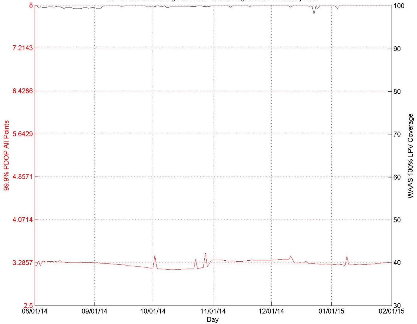
WAAS Conus Coverage vs PDOP Trends August 2014 to January 2015
