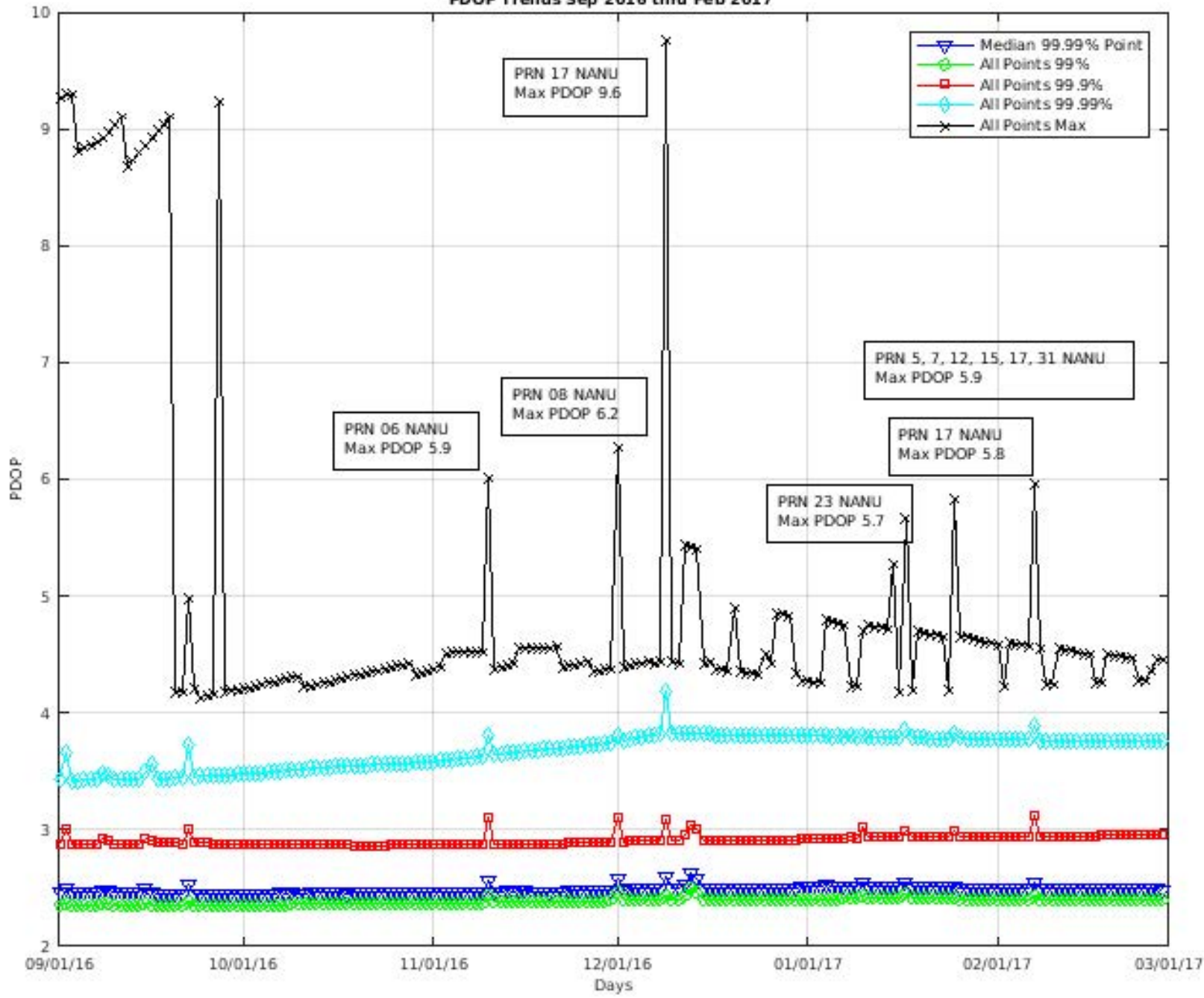
PDOP Trends Sep 2016 thru Feb 2017
