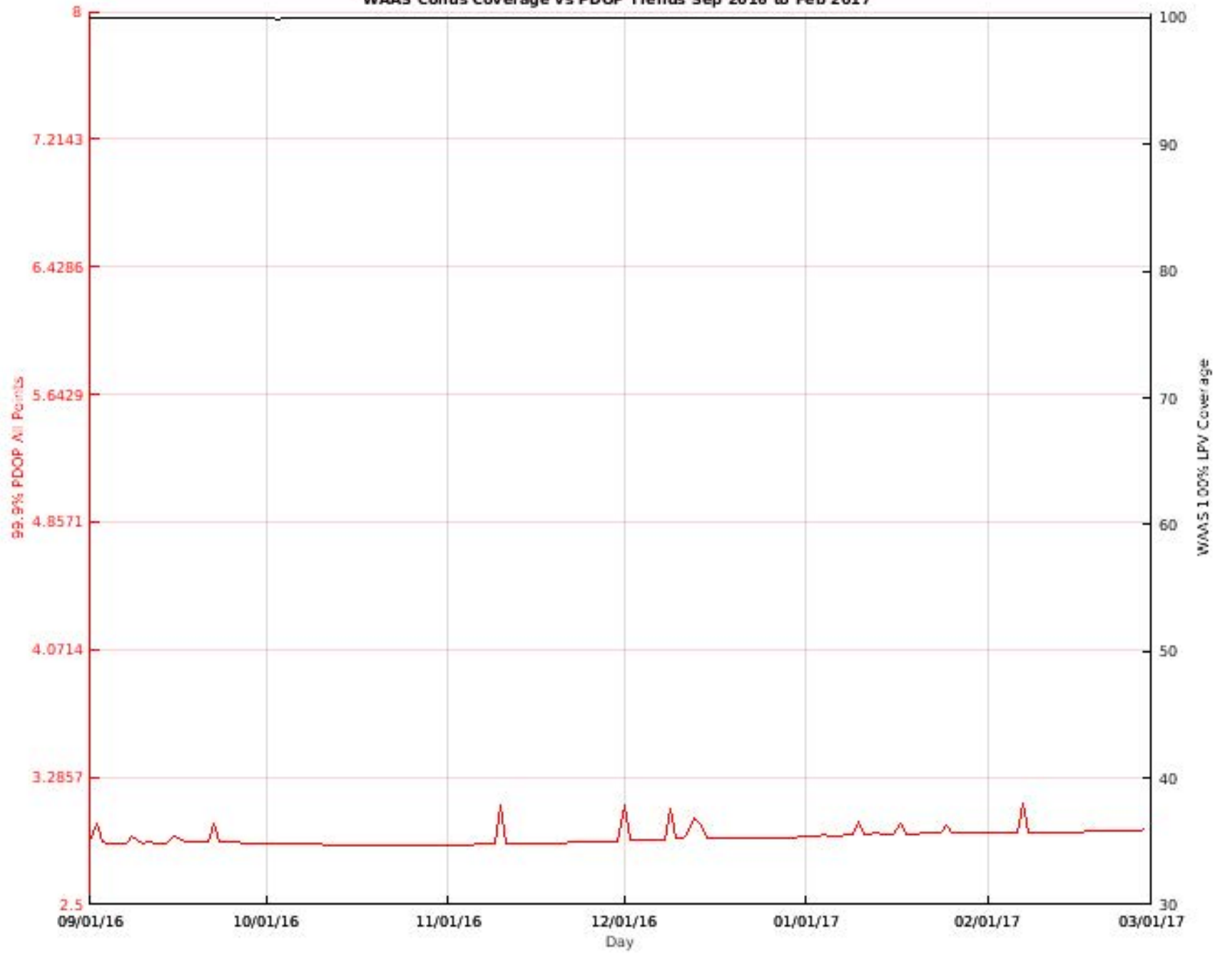
WAAS Conus Coverage vs PDOP Trends Sep 2016 to Feb 2017
