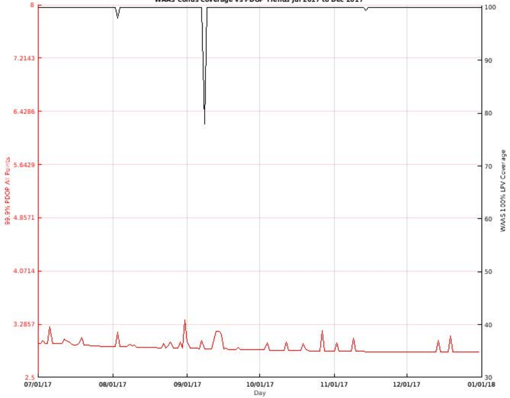
WAAS Conus Coverage vs PDOP Trends Jul 2017 to Dec 2017
