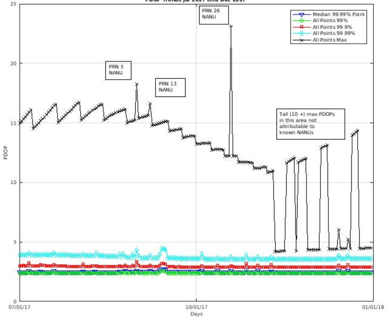
PDOP Trends Jul 2017 thru Dec 2017
