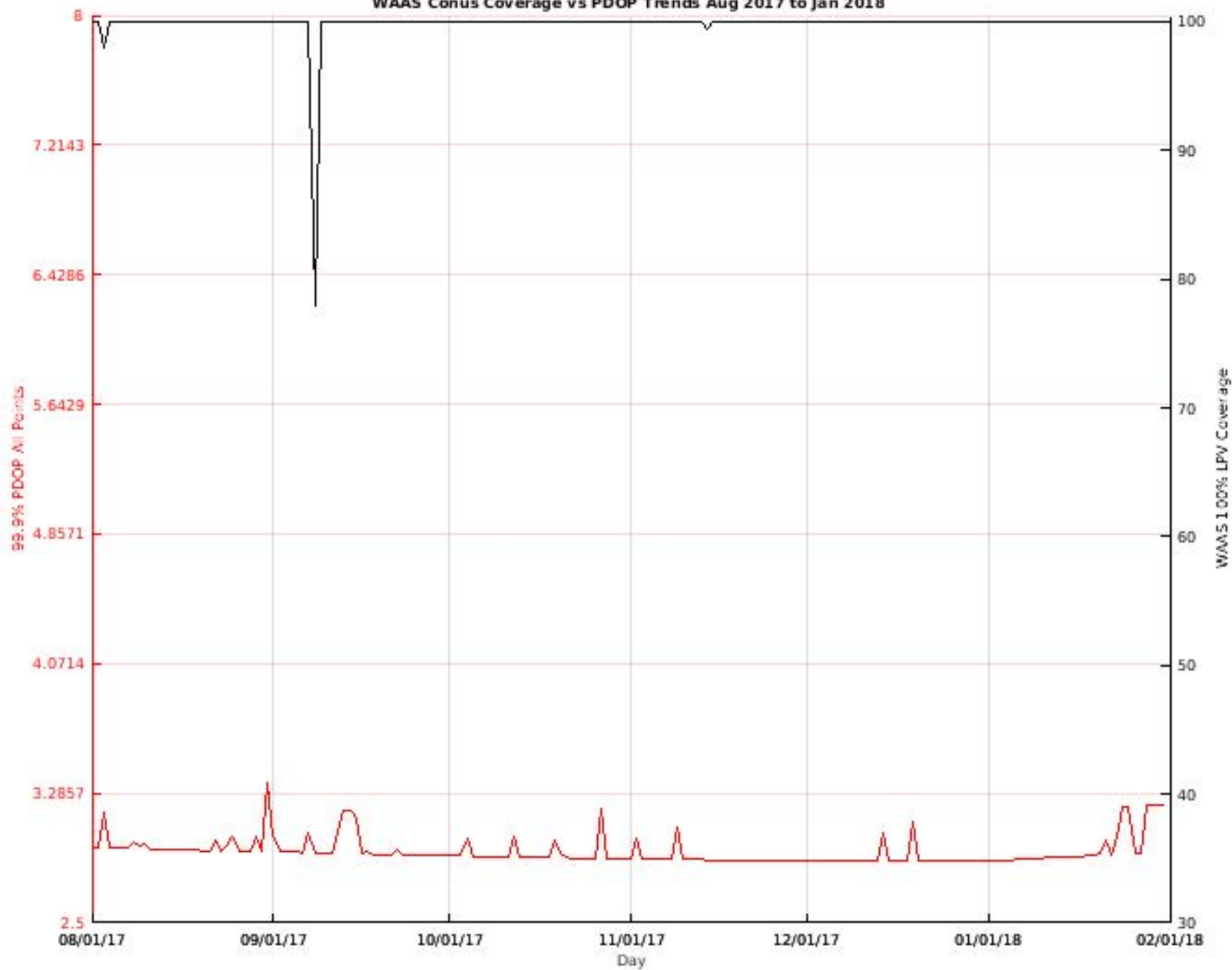
WAAS Conus Coverage vs PDOP Trends Aug 2017 to Jan 2018
