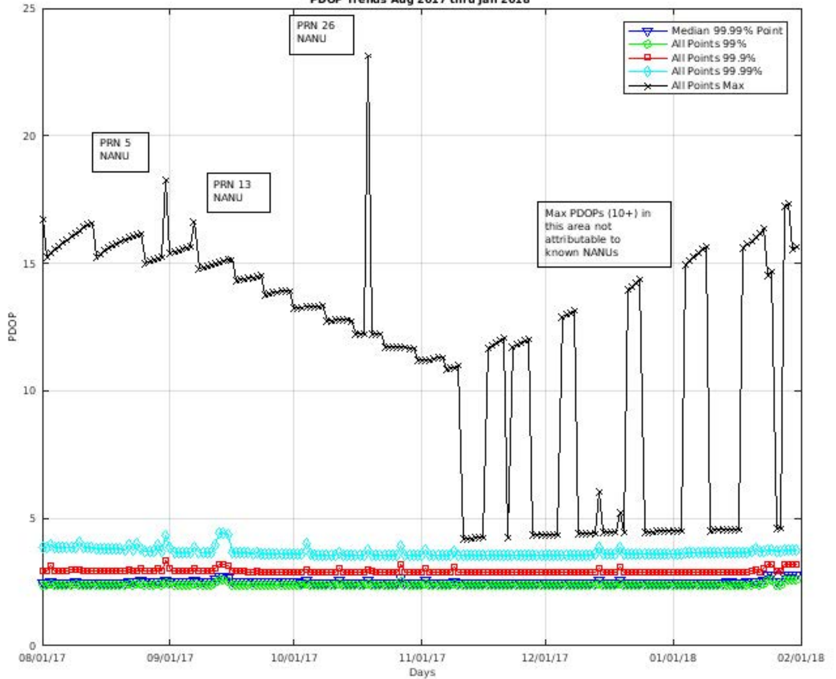
PDOP Trends Aug 2017 thru Jan 2018
