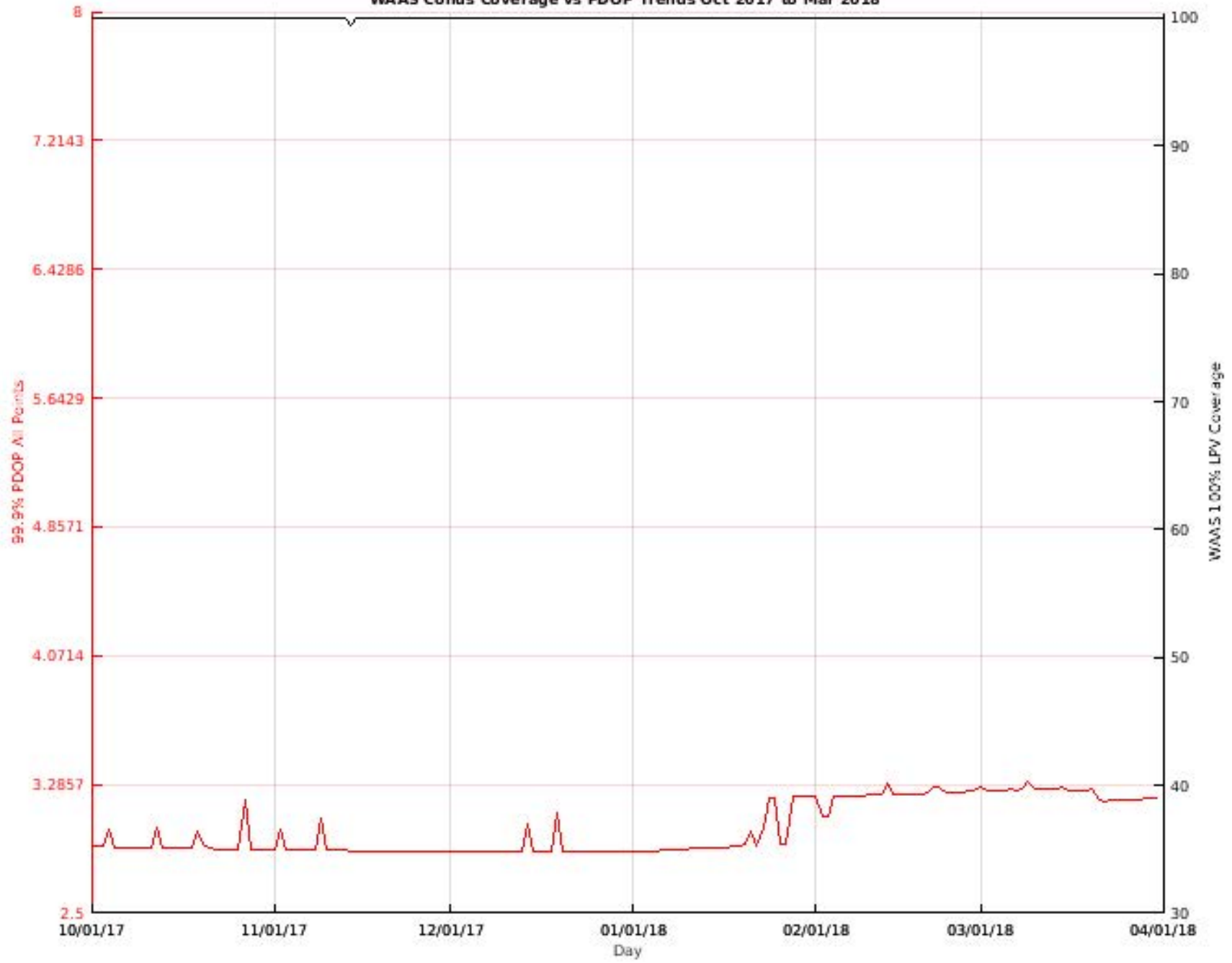
WAAS Conus Coverage vs PDOP Trends Oct 2017 to Mar 2018
