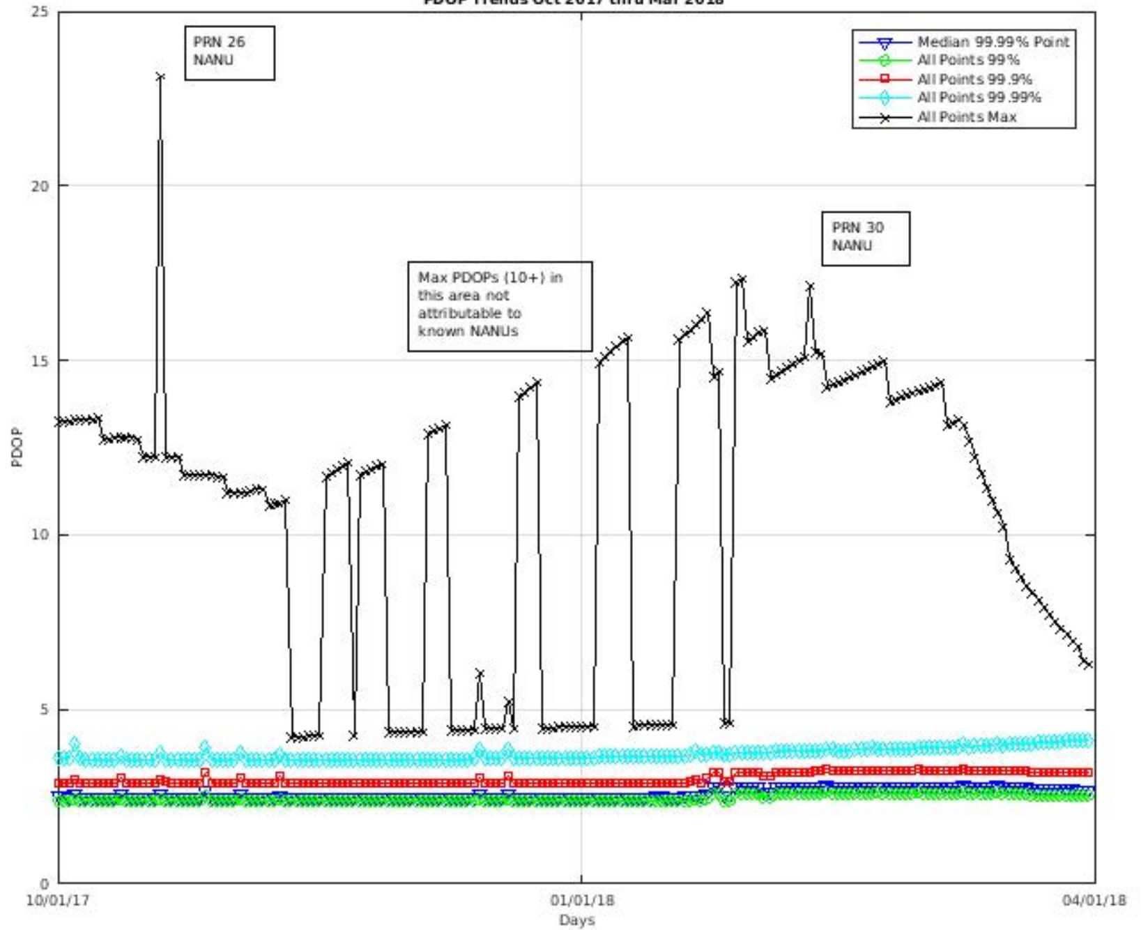
PDOP Trends Oct 2017 thru Mar 2018
