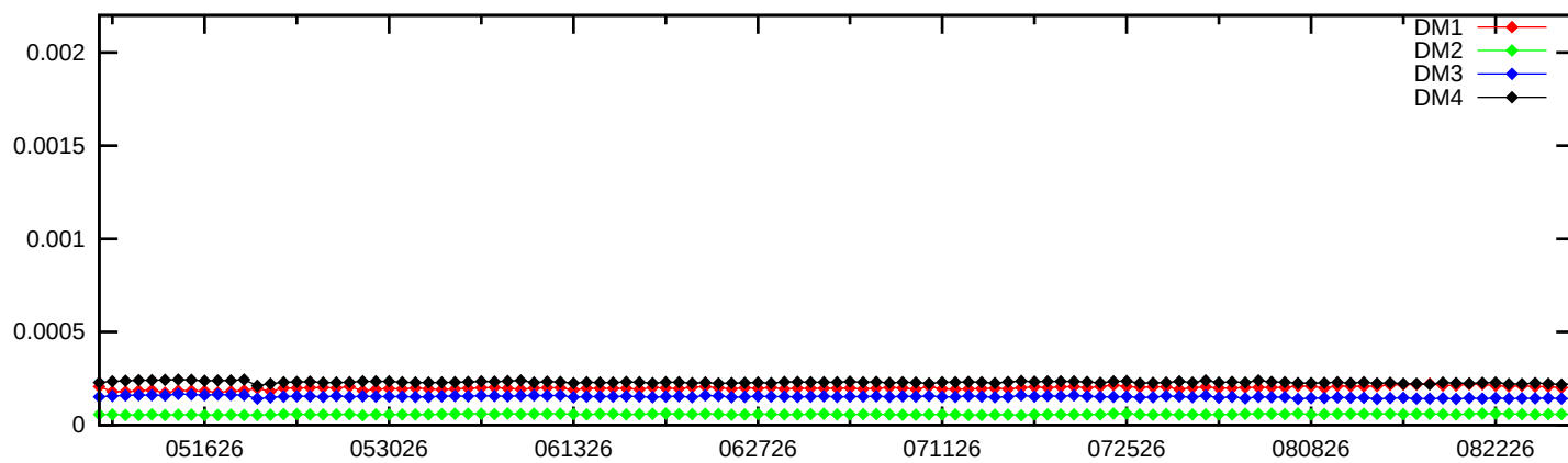
PRN 16 Bias (Daily average)
