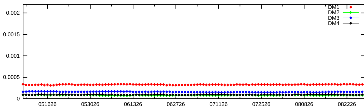
PRN 31 Bias (Daily average)
