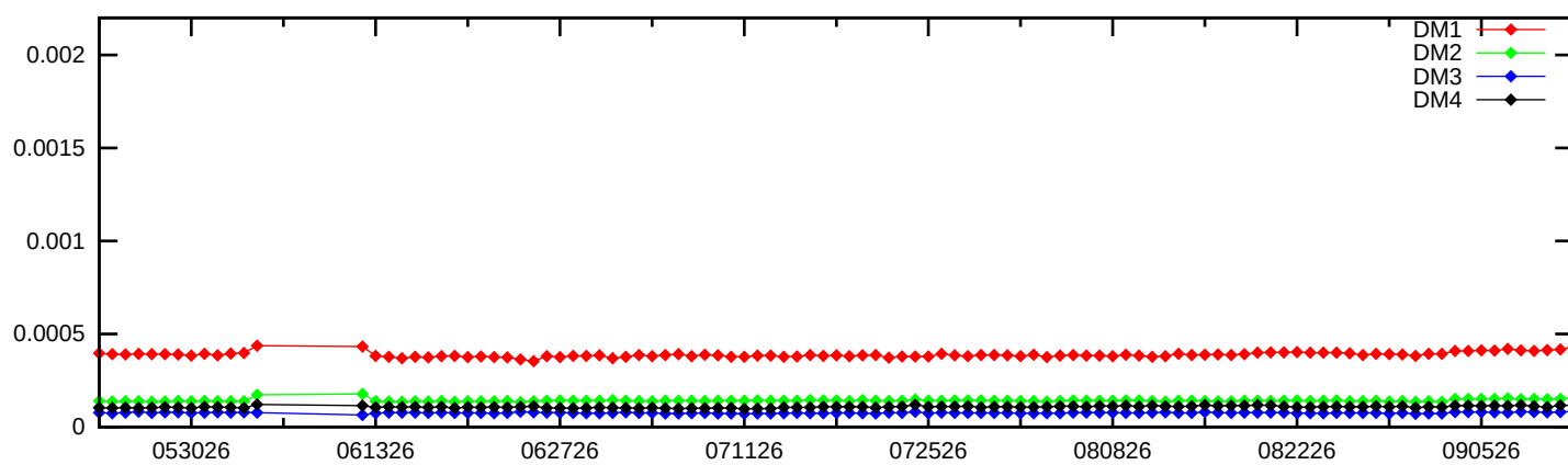
PRN 18 Bias (Daily average)
