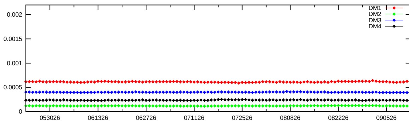
PRN 19 Bias (Daily average)
