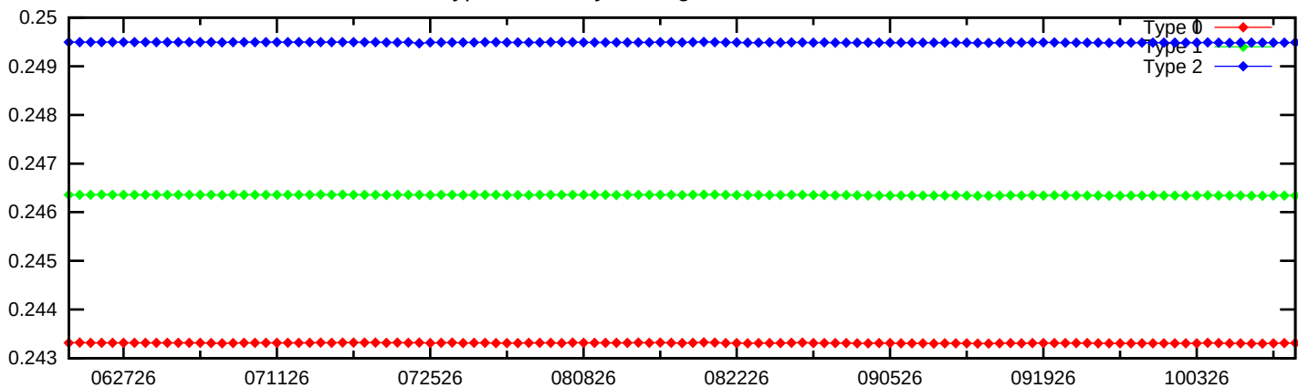
Type Bias Daily Average, Detection Metrics 3
