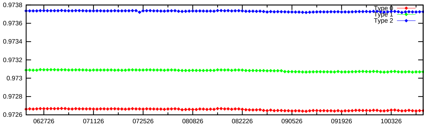
Type Bias Daily Average, Detection Metrics 4
