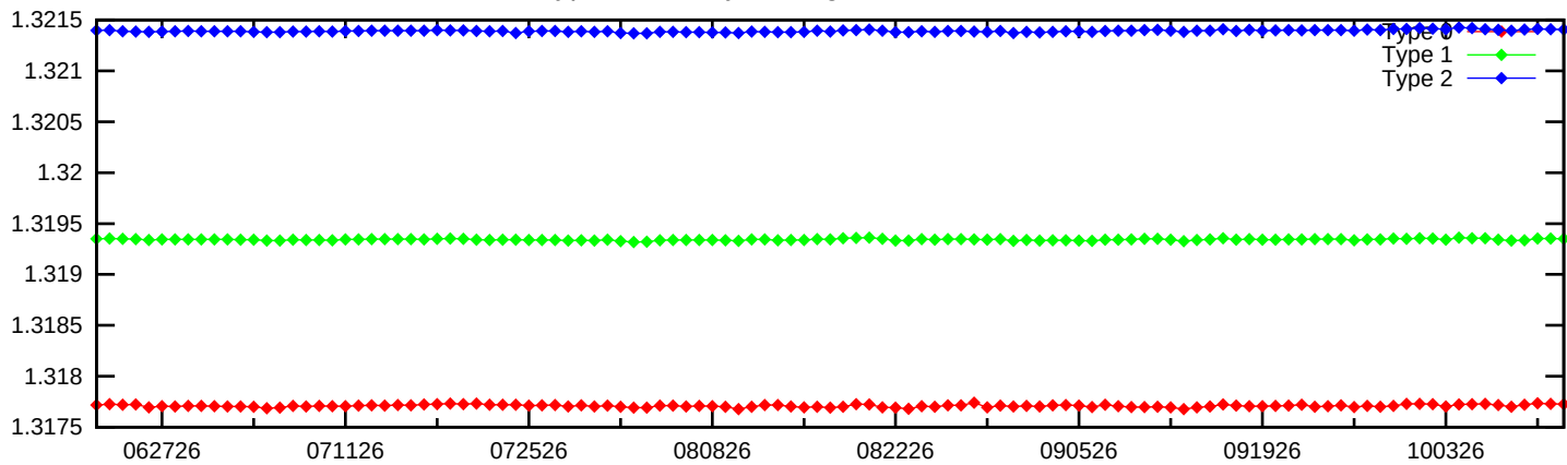
Type Bias Daily Average, Detection Metrics 2
