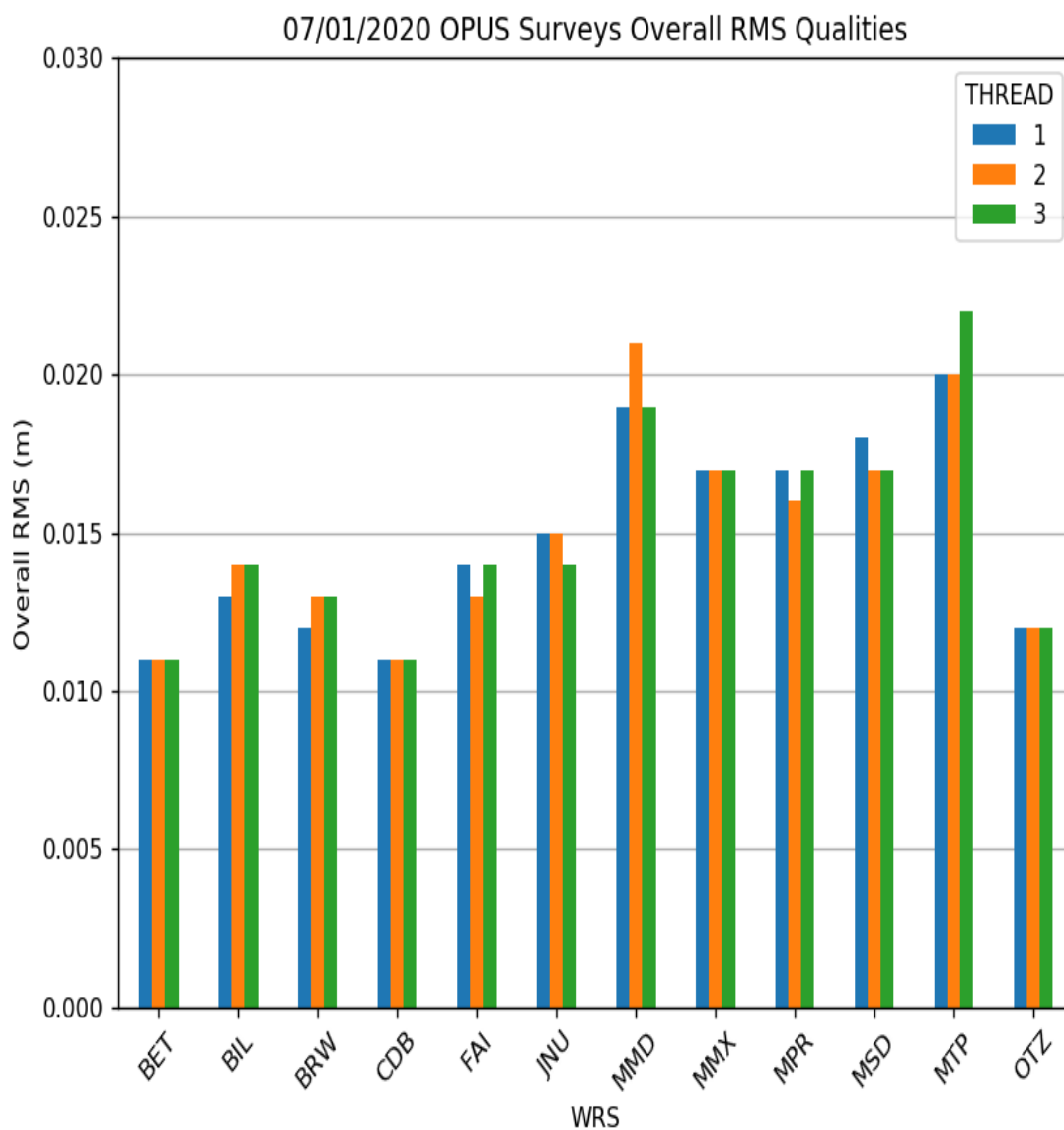
Figure 10-4 OPUS Survey Overall RMS Qualities
