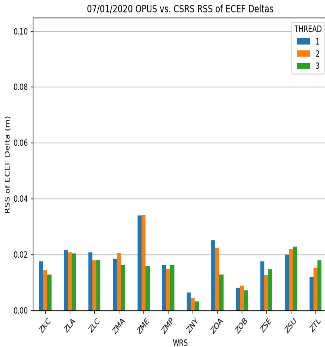
Figure 10-9 OPUS vs. CSRS RSS ECEF Deltas
