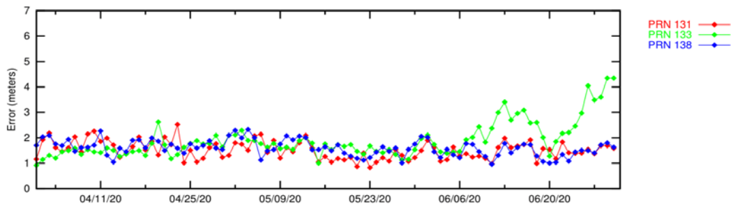
Figure 6-3. Range Error (PRN131, PRN133, PRN138)–Washington D.C.
