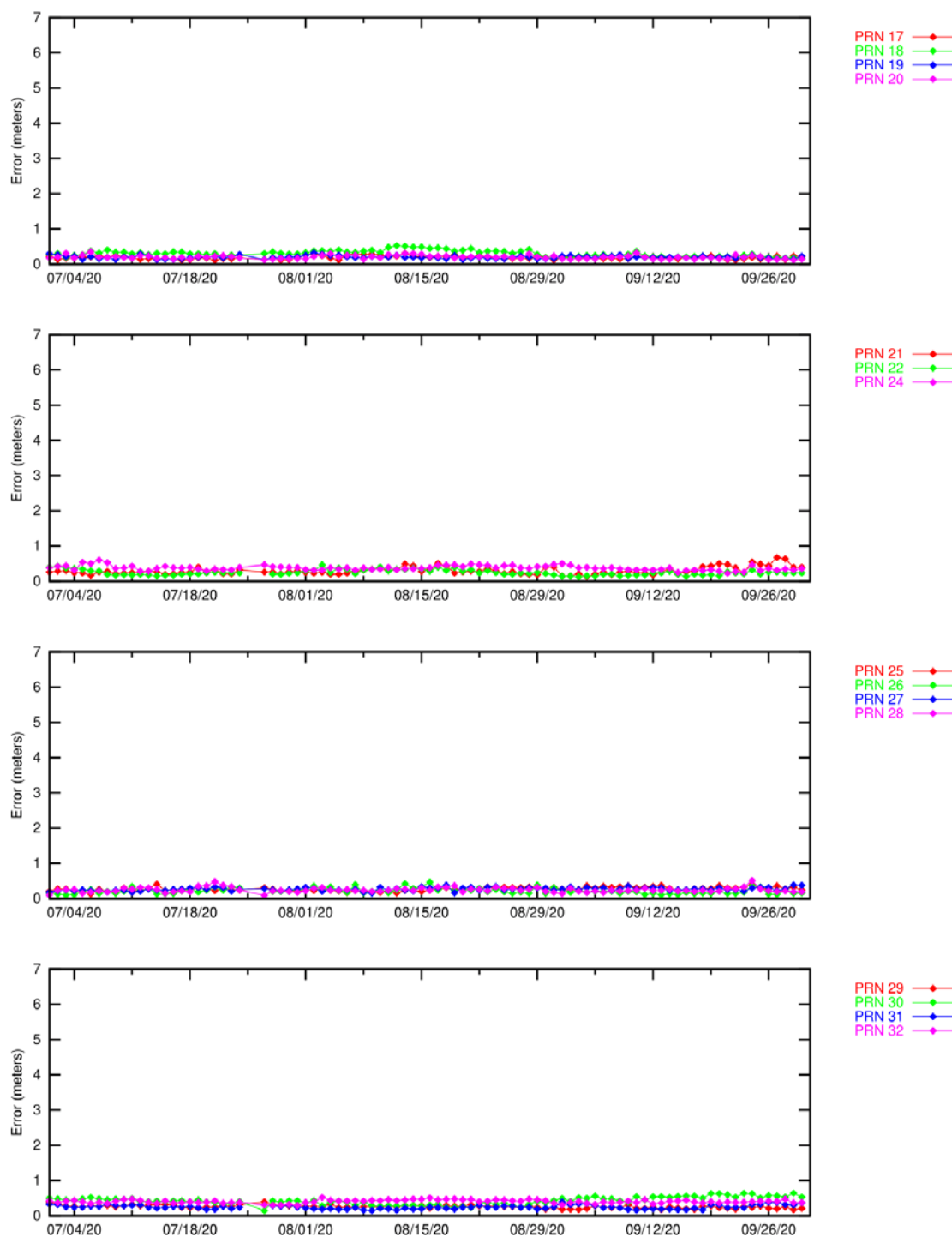
Figure 6-5. Ionospheric Error (PRN17–PRN32)–Washington D.C.
