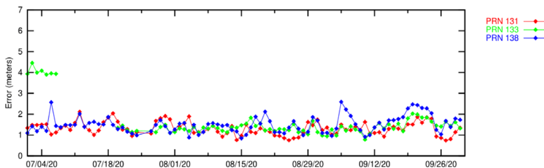
Figure 6-3. Range Error (PRN131, PRN133, PRN 138)–Washington D.C.
