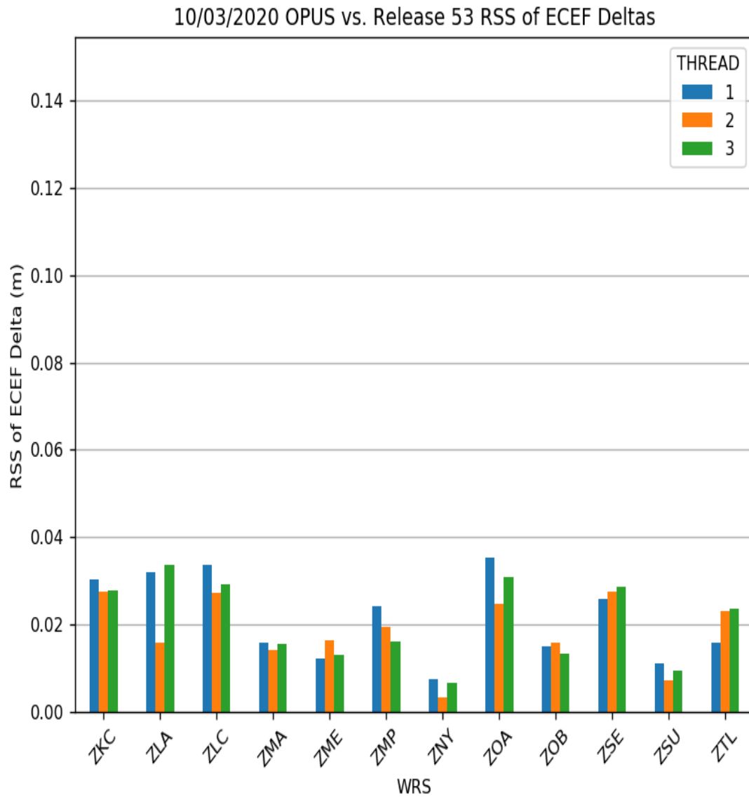
Figure 10-3. Build WE7.164c Antenna Positions Deltas OPUS Survey
