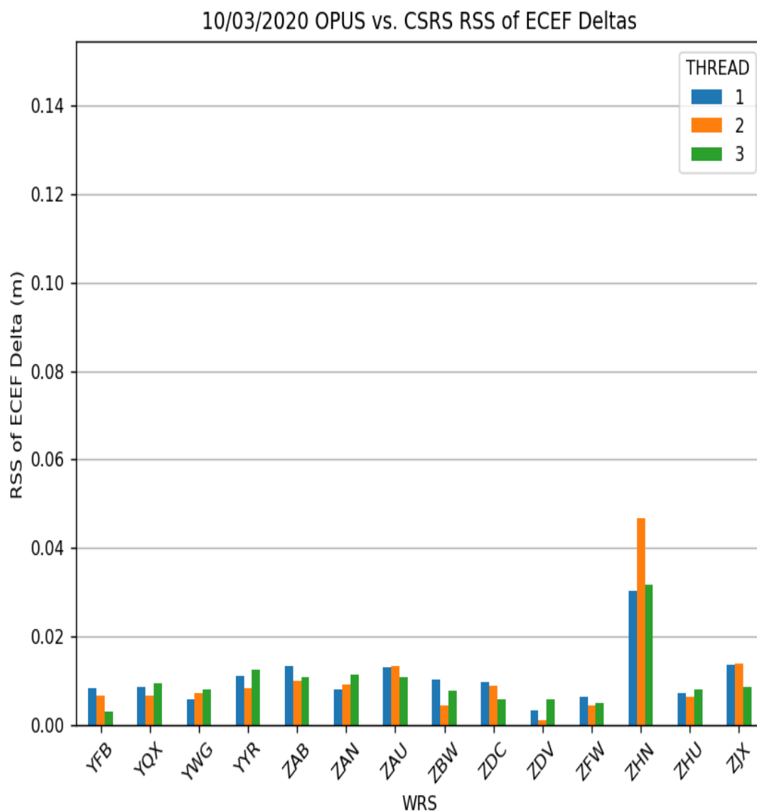
Figure 10-8. OPUS vs. CSRS RSS ECEF Deltas
