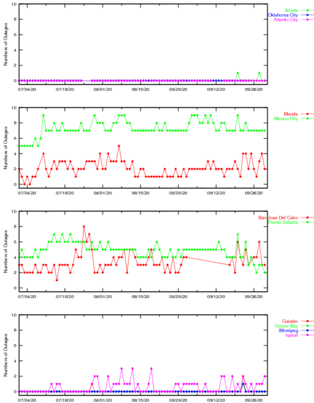
Figure 3-12. LPV200 Outages
