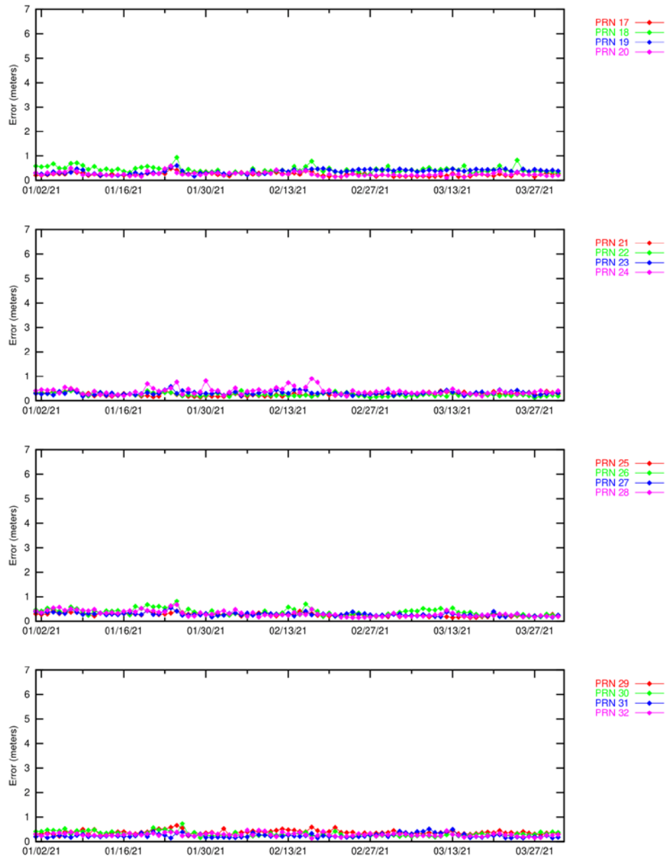
Figure 6-5 Ionospheric Error (PRN17 – PRN32) – Washington D.C.
