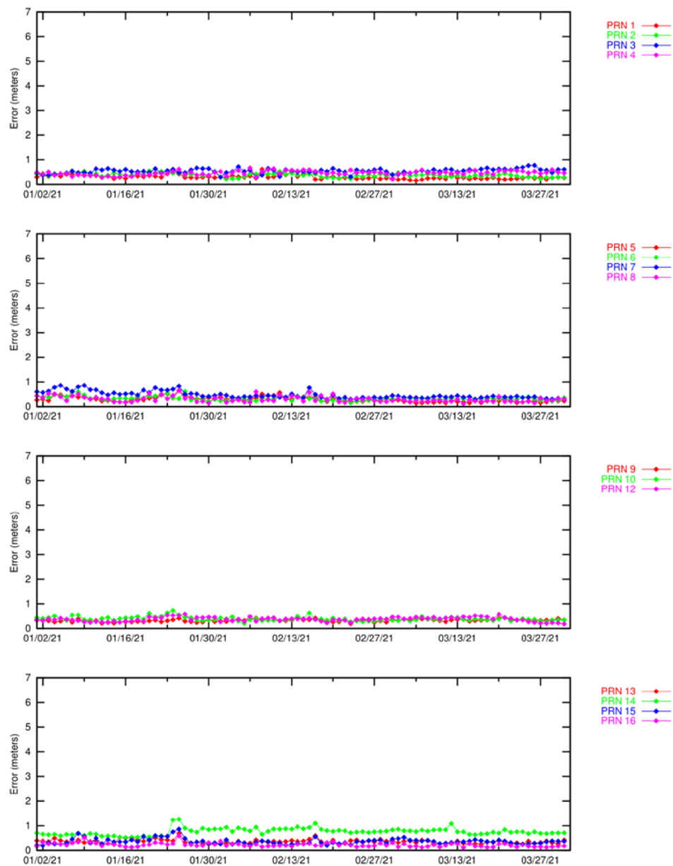
Figure 6-4 Ionospheric Error (PRN1 – PRN16) – Washington D.C.
