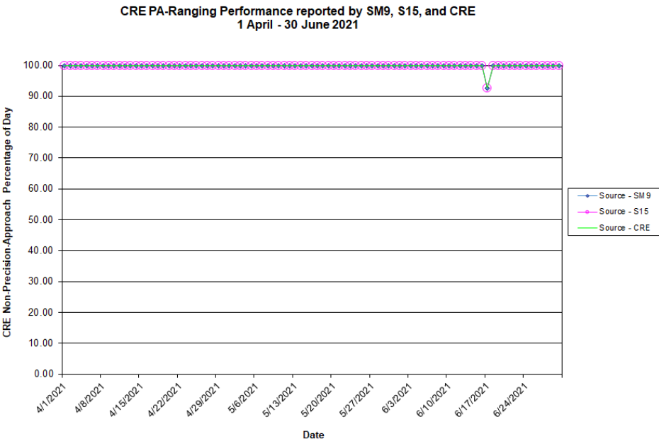
Figure 7-3 Daily PA CRE GEO Ranging Availability Trend
