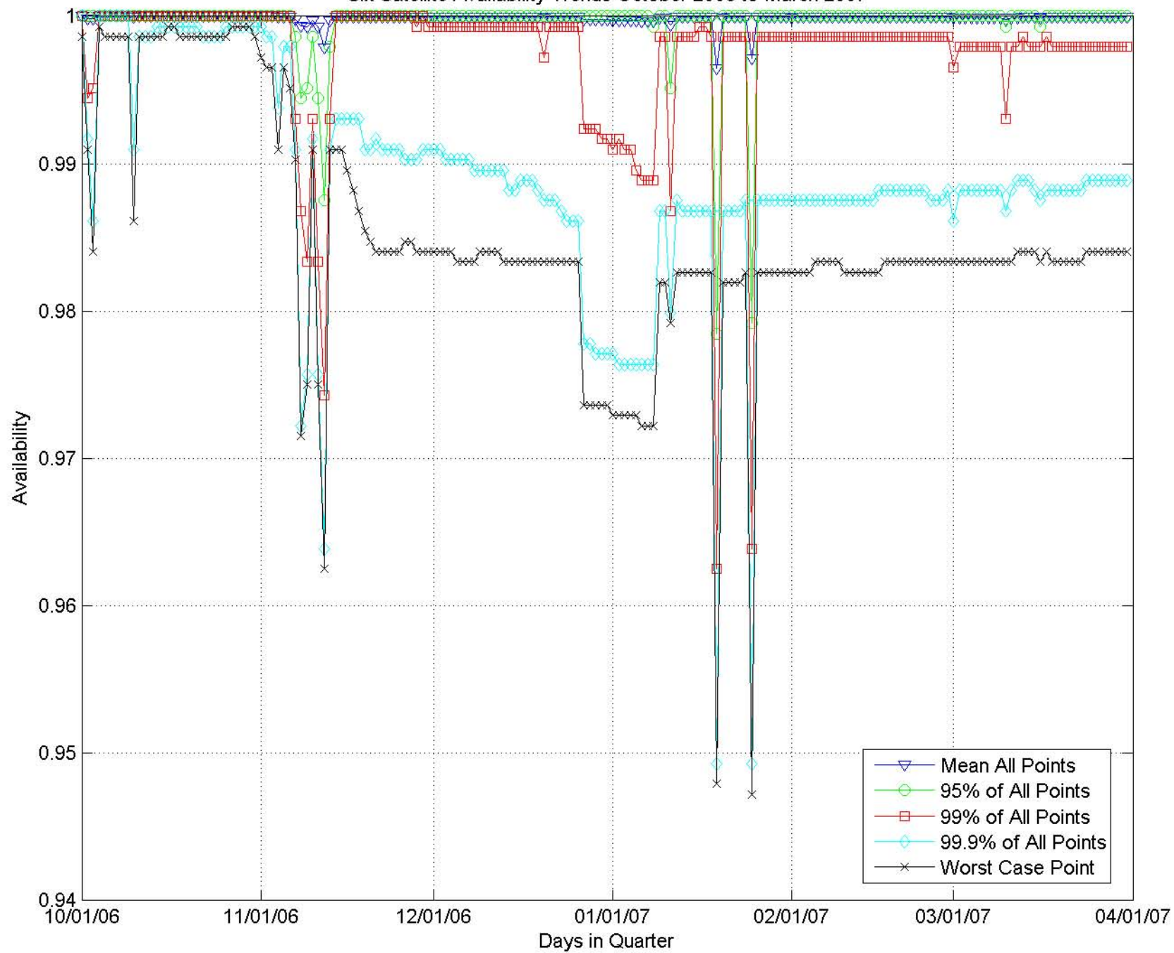
Six Satellite Availability Trends October 2006 to March 2007
