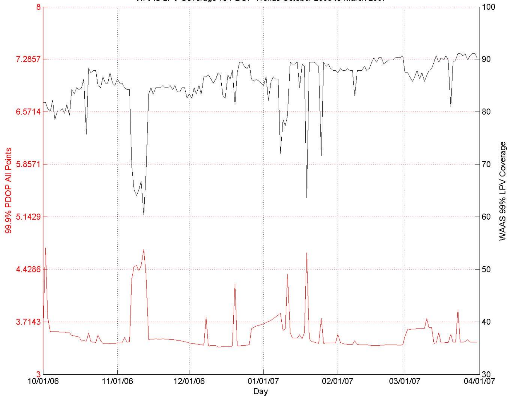
WAAS LPV Coverage vs PDOP Trends October 2006 to March 2007
