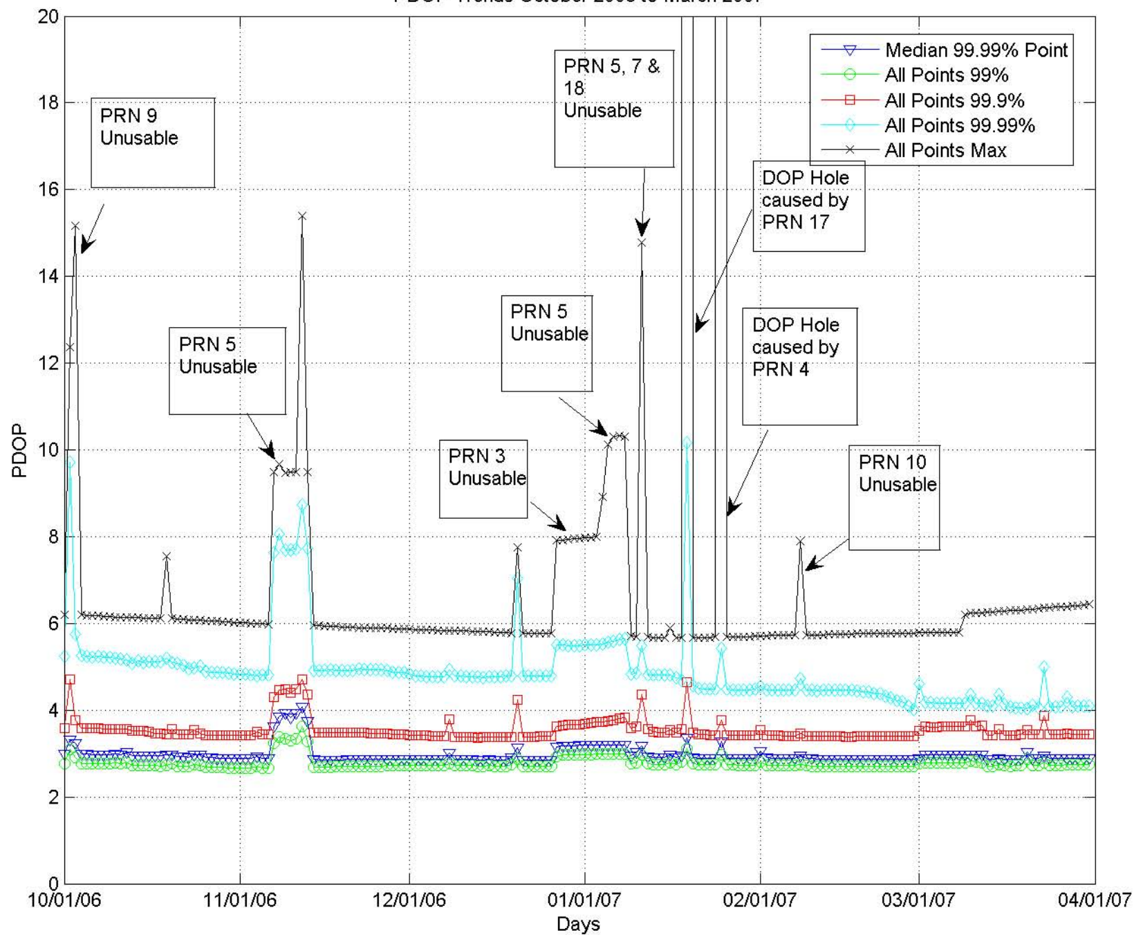
PDOP Trends October 2006 to March 2007
