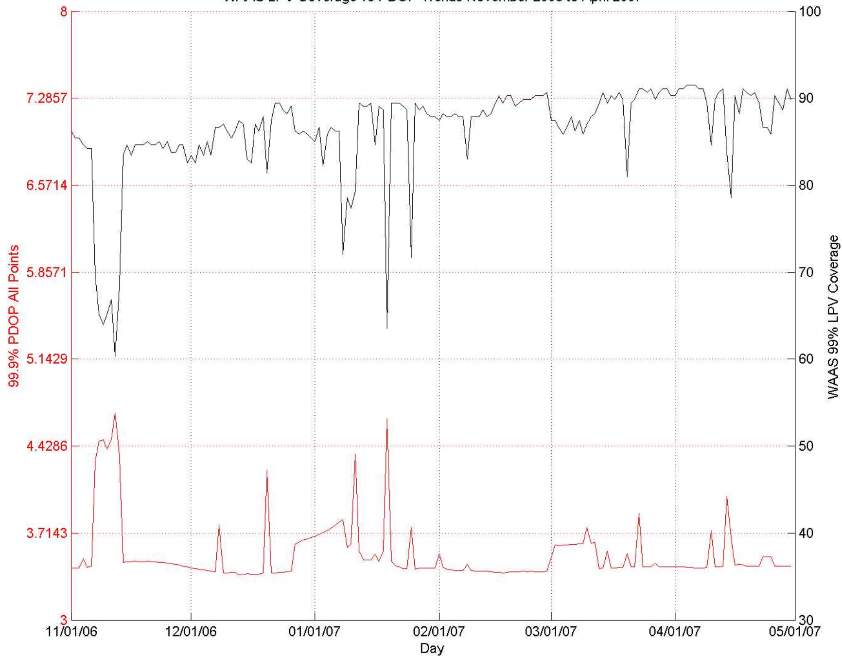
WAAS LPV Coverage vs PDOP Trends November 2006 to April 2007
