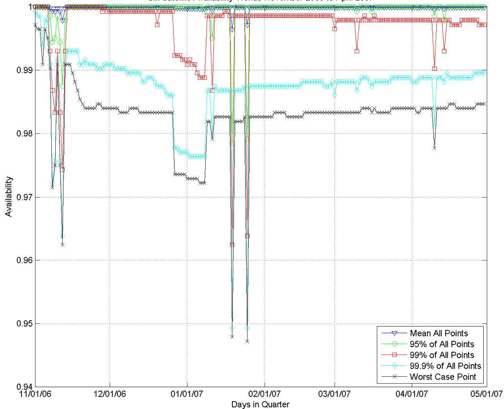
Six Satellite Availability Trends November 2006 to April 2007
