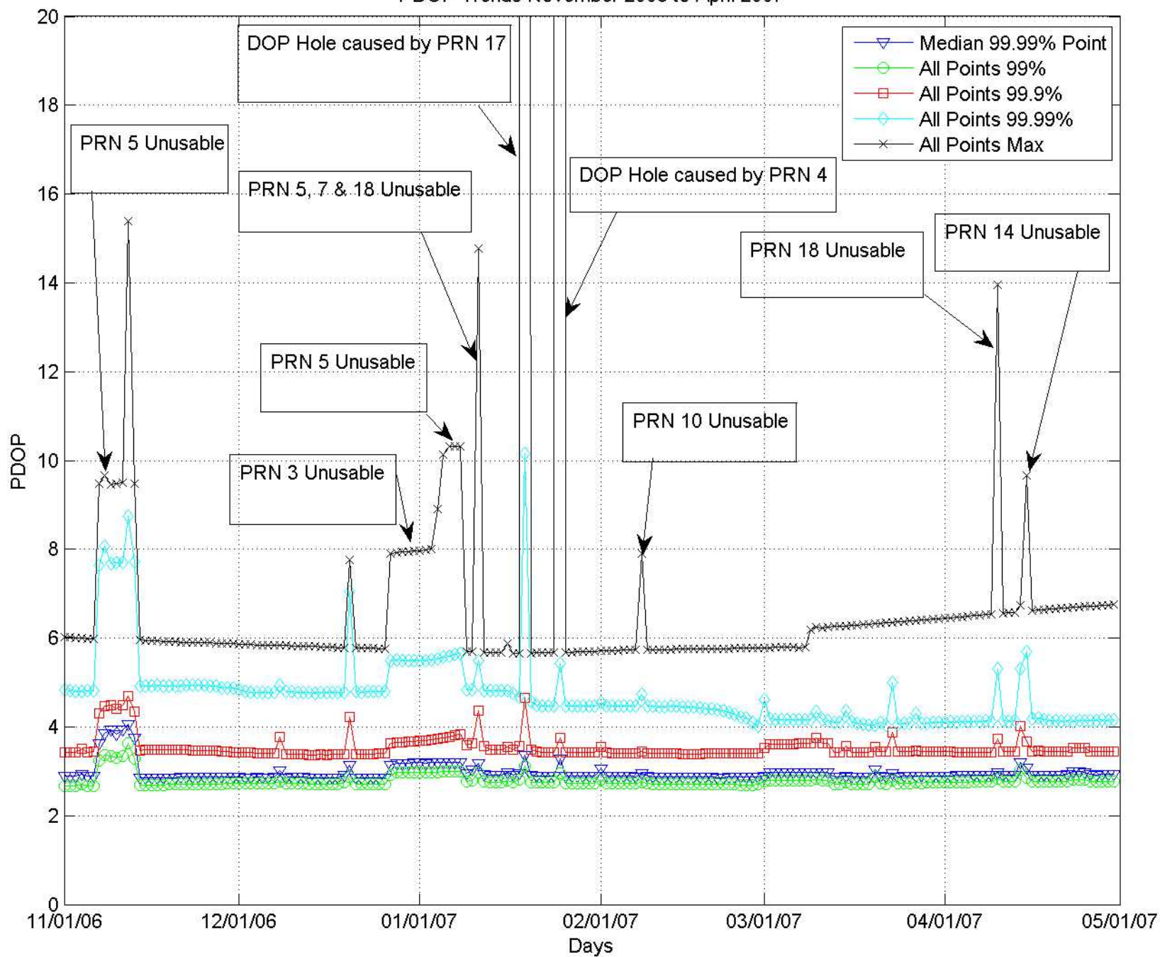
PDOP Trends November 2006 to April 2007
