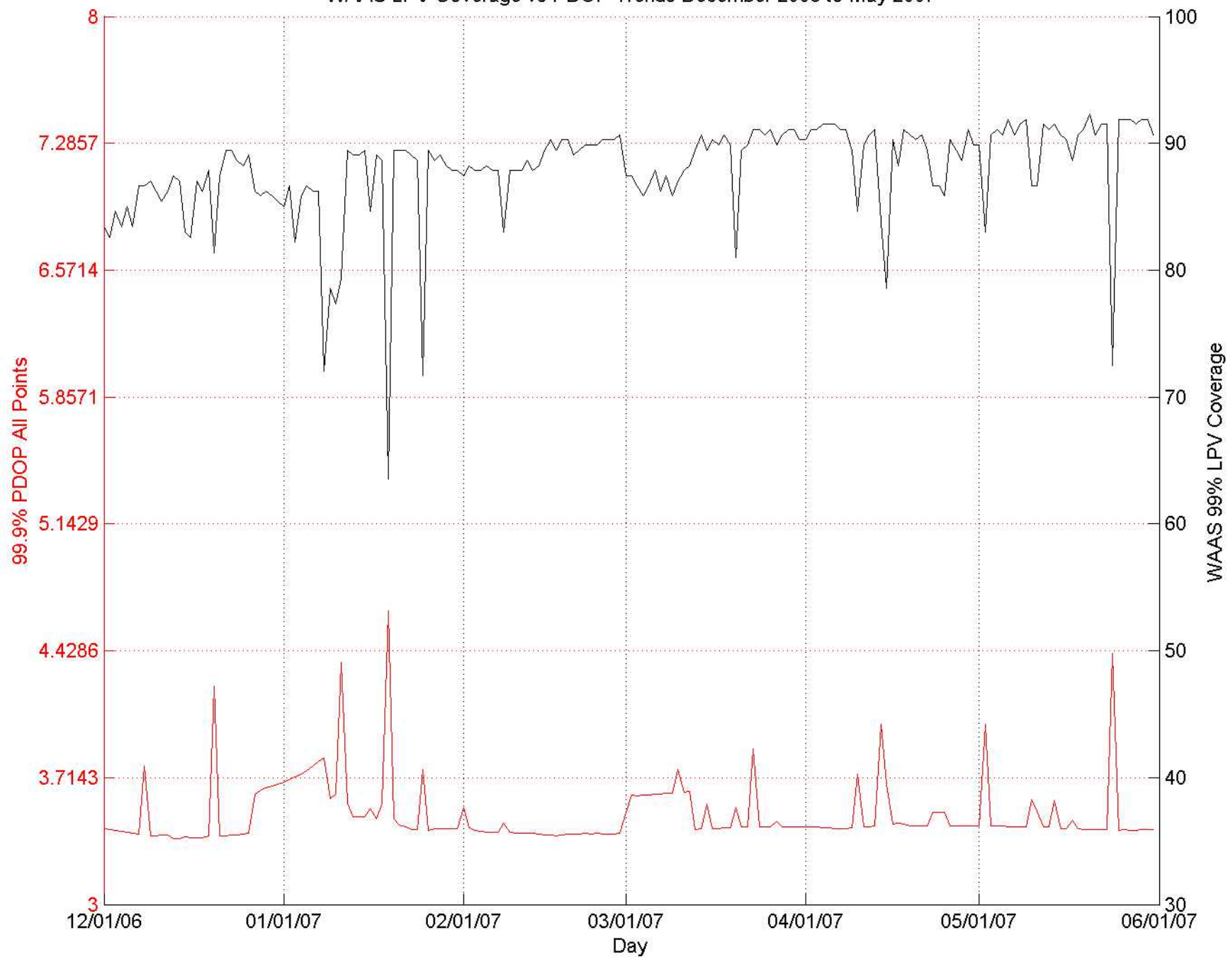
WAAS LPV Coverage vs PDOP Trends December 2006 to May 2007
