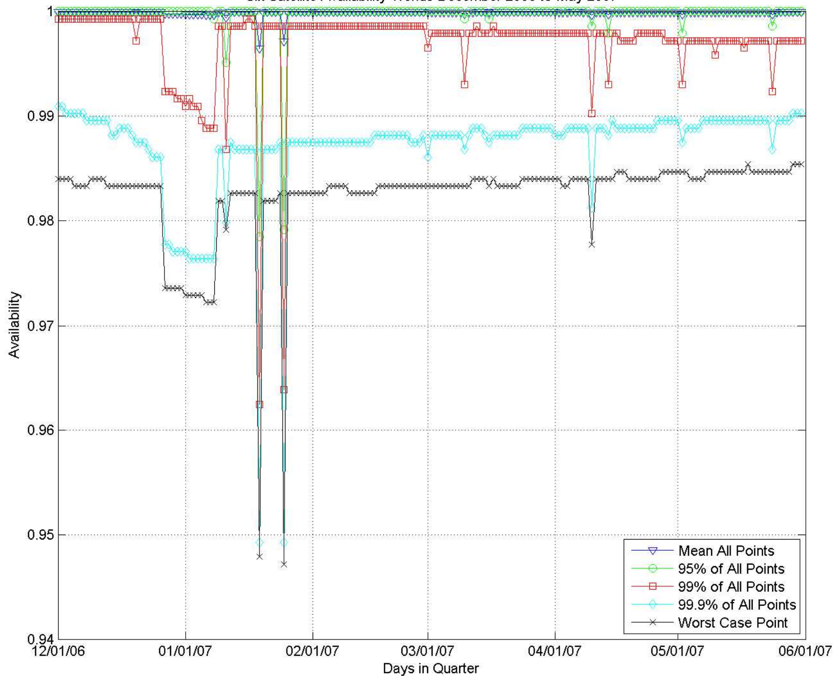
Six Satellite Availability Trends December 2006 to May 2007
