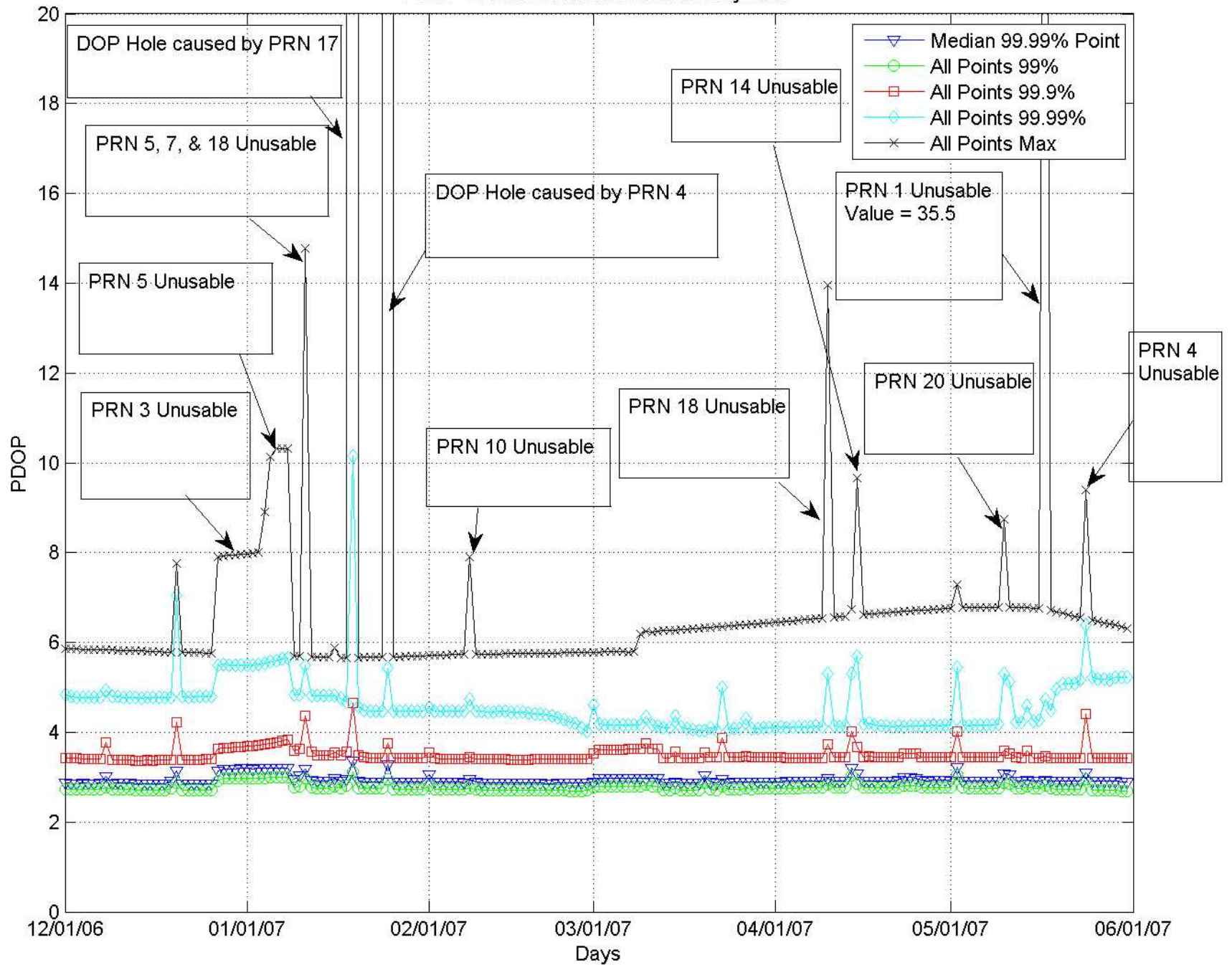
PDOP Trends December 2006 to May 2007
