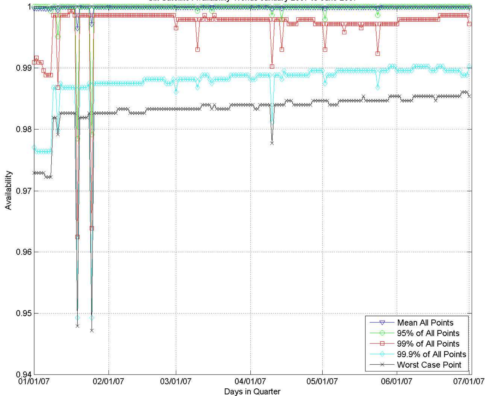
Six Satellite Availability Trends January 2007 to June 2007
