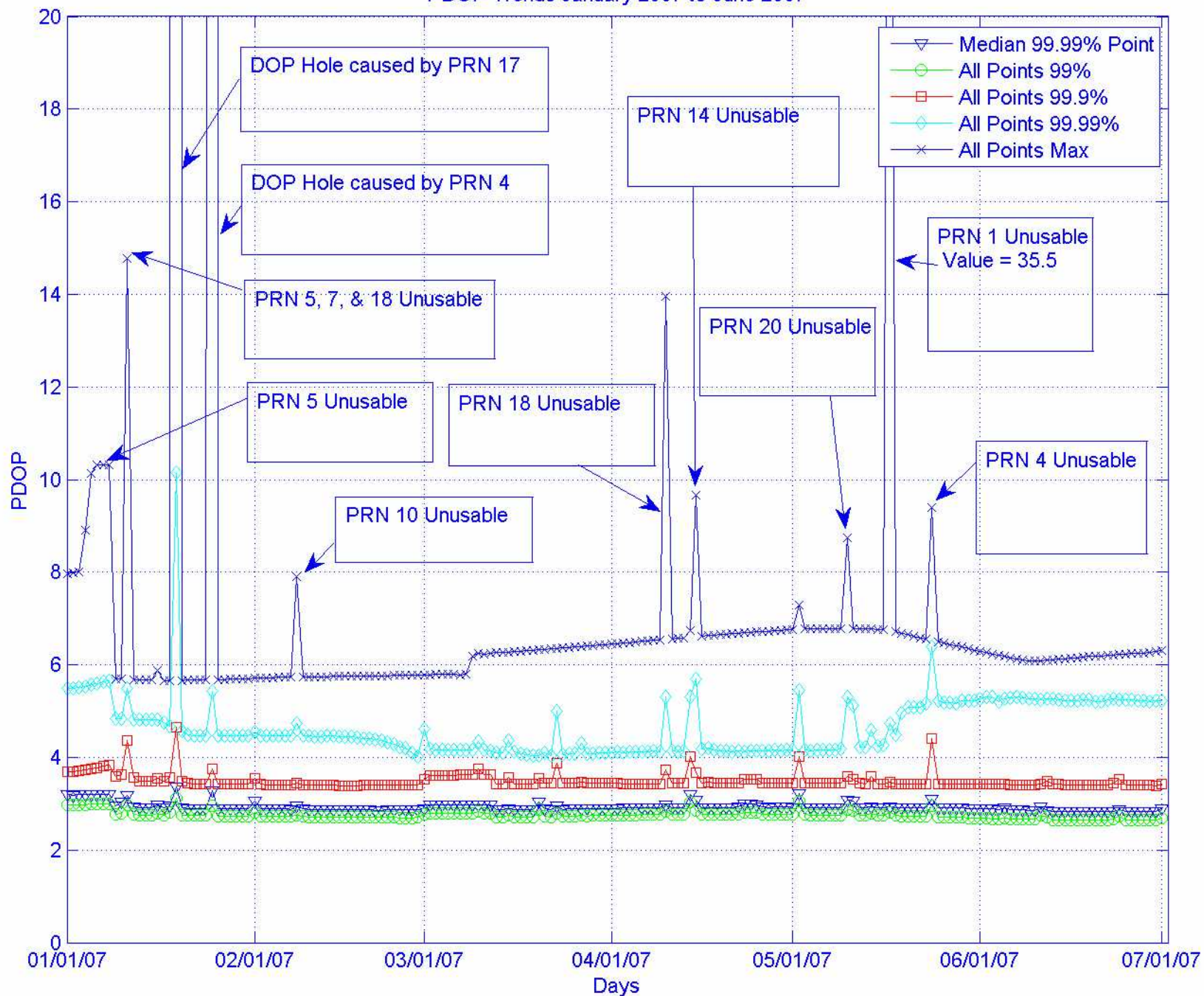
PDOP Trends January 2007 to June 2007
