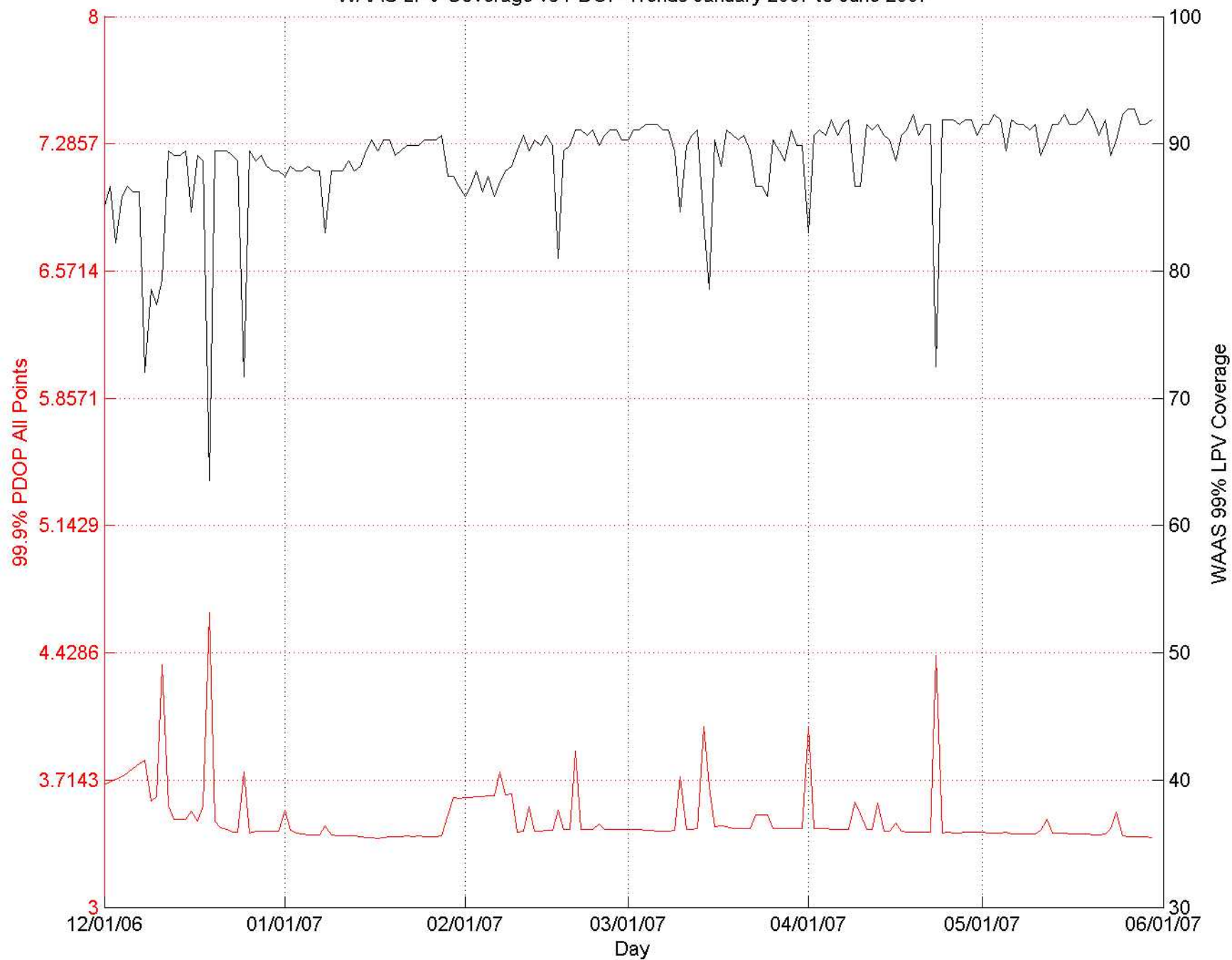
WAAS LPV Coverage vs PDOP Trends January 2007 to June 2007
