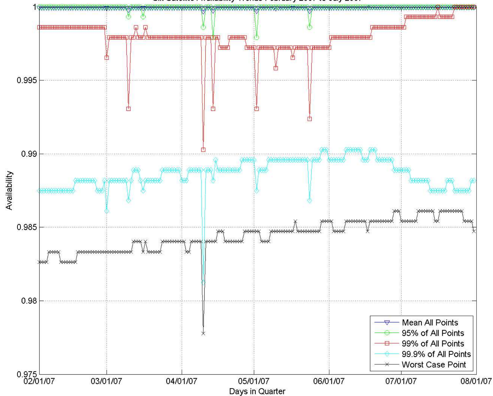
Six Satellite Availability Trends February 2007 to July 2007
