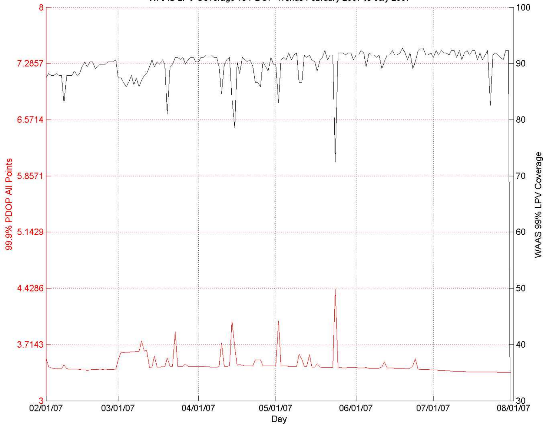
WAAS LPV Coverage vs PDOP Trends February 2007 to July 2007
