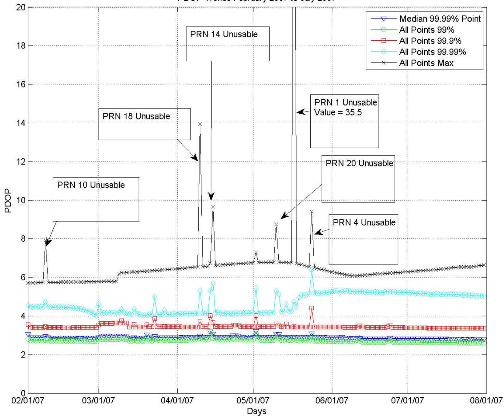
PDOP Trends February 2007 to July 2007
