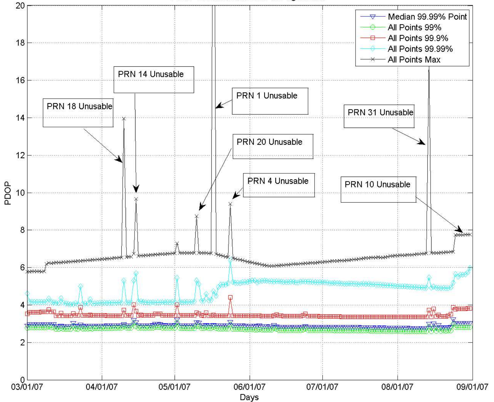
PDOP Trends March 2007 to August 2007
