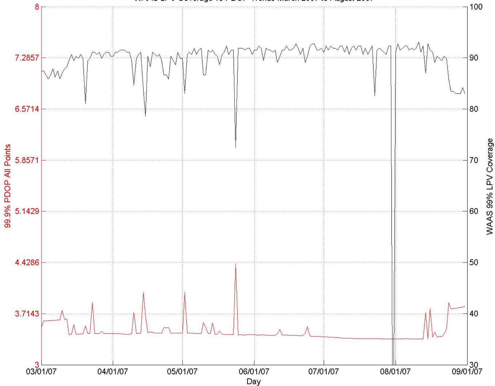
WAAS LPV Coverage vs PDOP Trends March 2007 to August 2007
