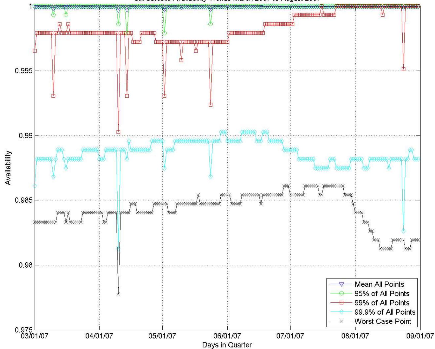
Six Satellite Availability Trends March 2007 to August 2007
