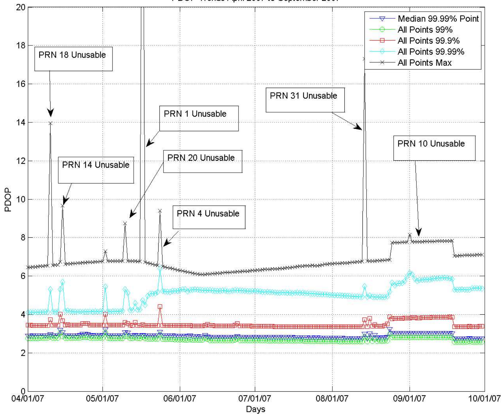
PDOP Trends April 2007 to September 2007
