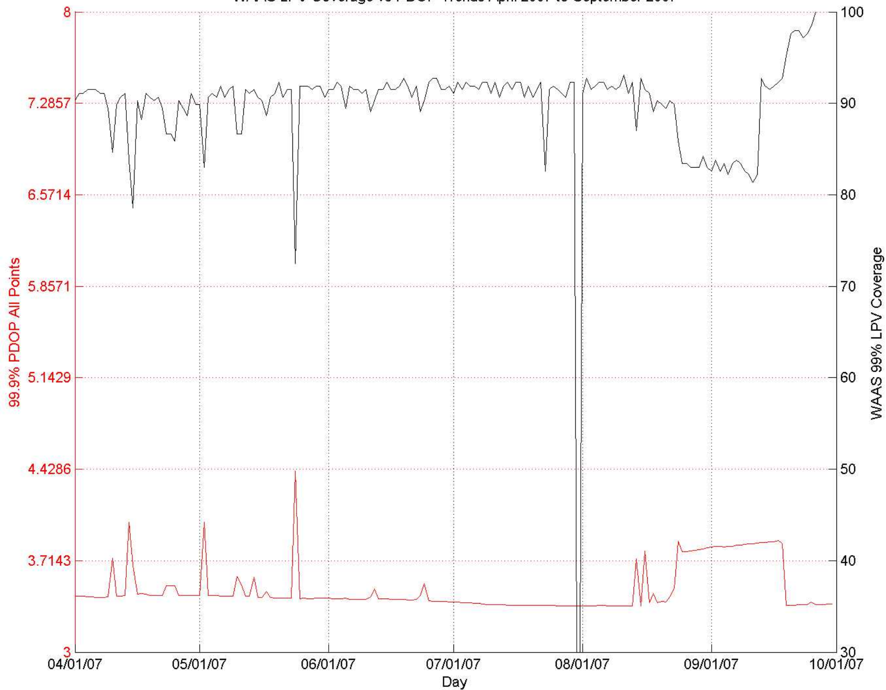
WAAS LPV Coverage vs PDOP Trends April 2007 to September 2007
