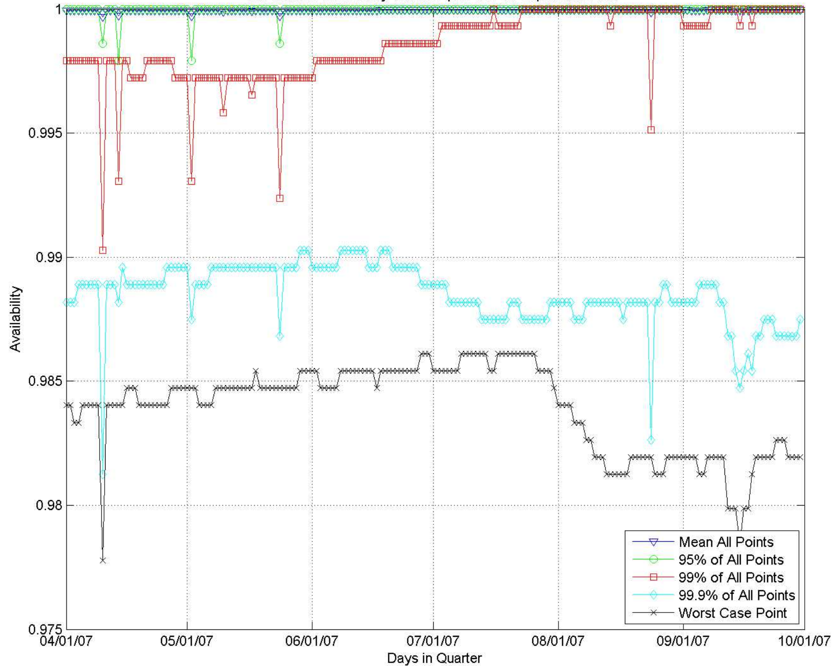
Six Satellite Availability Trends April 2007 to September 2007
