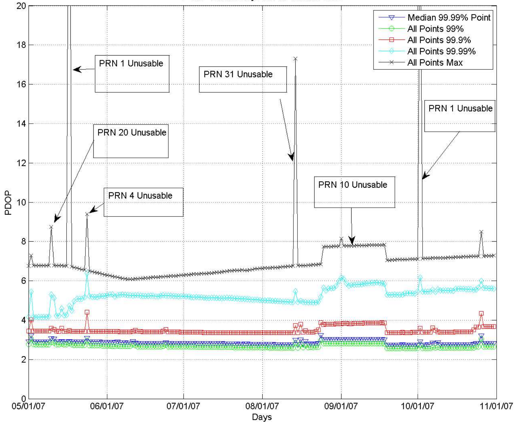
PDOP Trends May 2007 to October 2007
