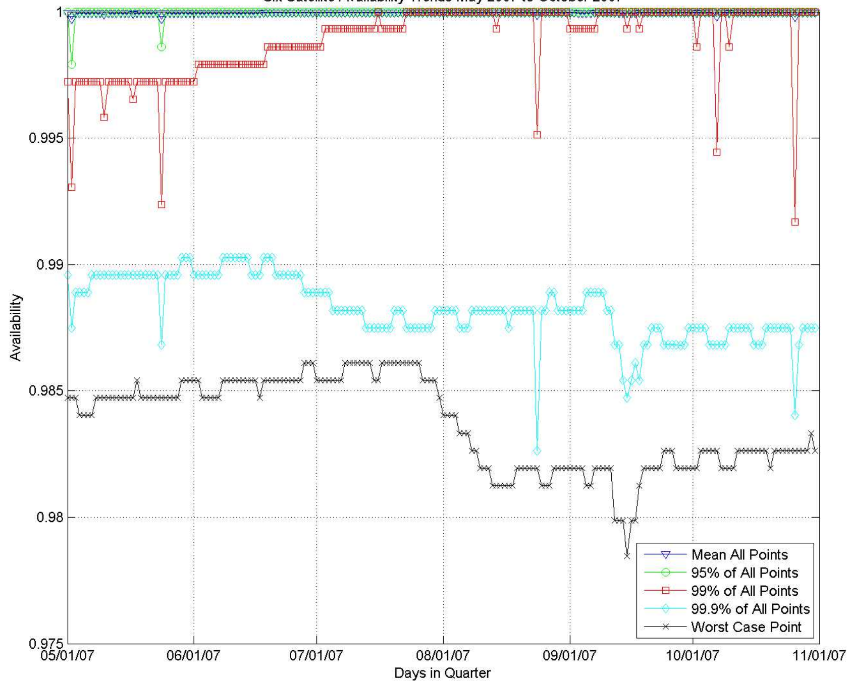
Six Satellite Availability Trends May 2007 to October 2007
