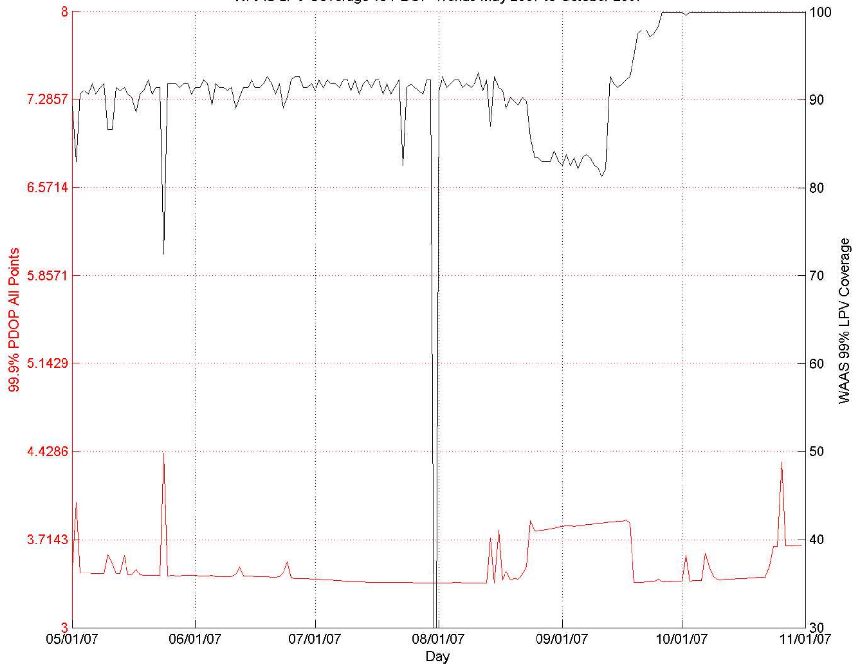
WAAS LPV Coverage vs PDOP Trends May 2007 to October 2007
