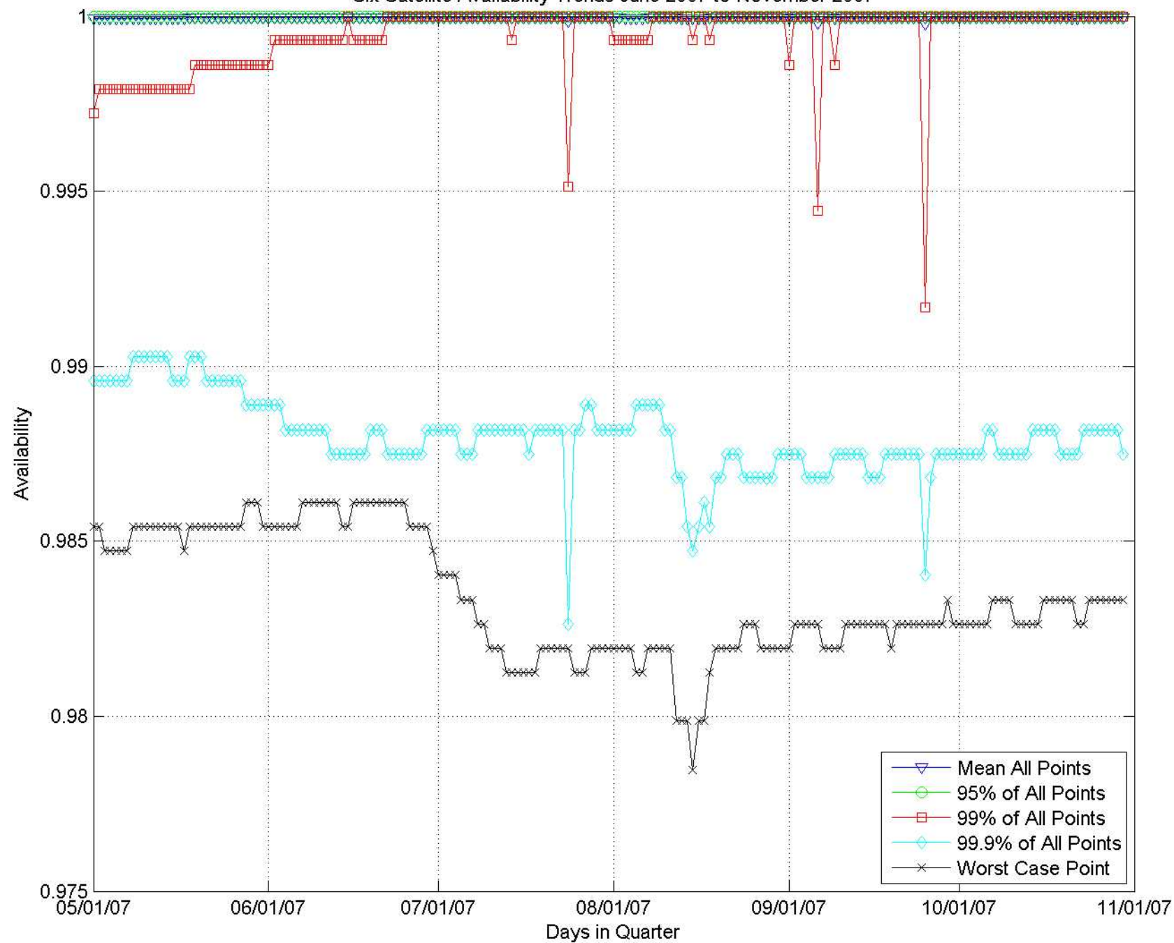
Six Satellite Availability Trends June 2007 to November 2007
