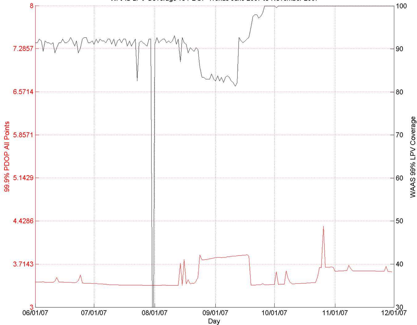
WAAS LPV Coverage vs PDOP Trends June 2007 to November 2007
