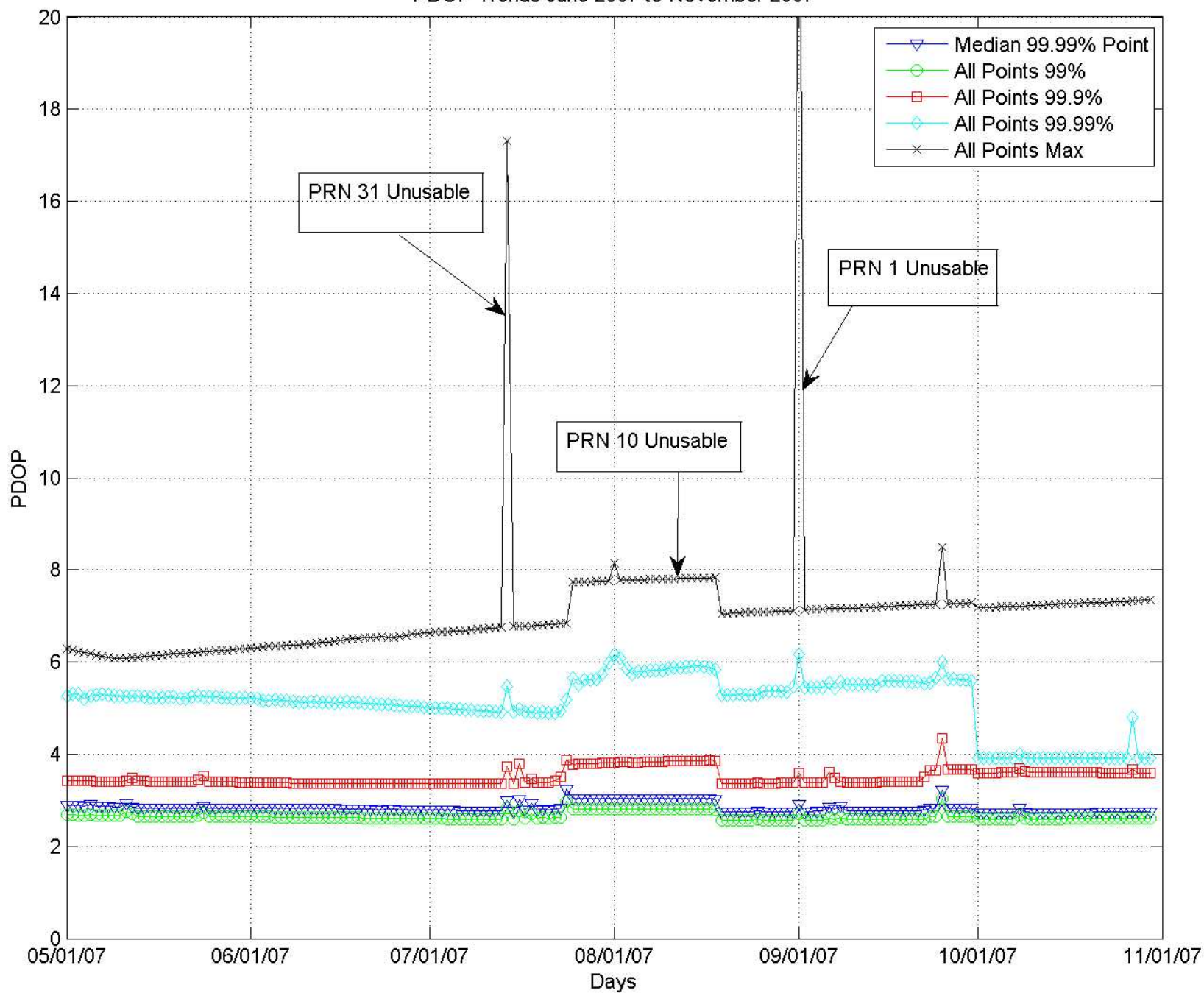
PDOP Trends June 2007 to November 2007
