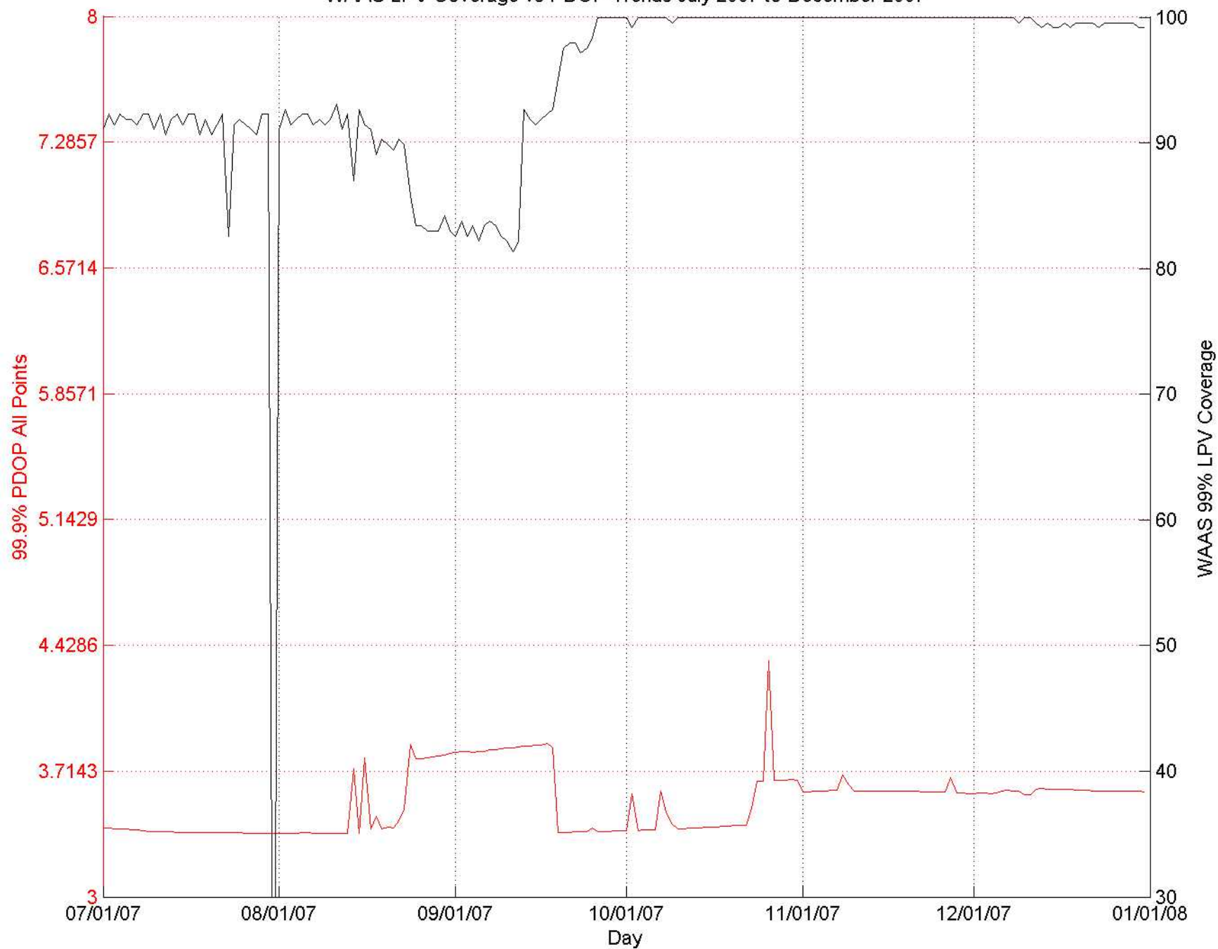
WAAS LPV Coverage vs PDOP Trends July 2007 to December 2007
