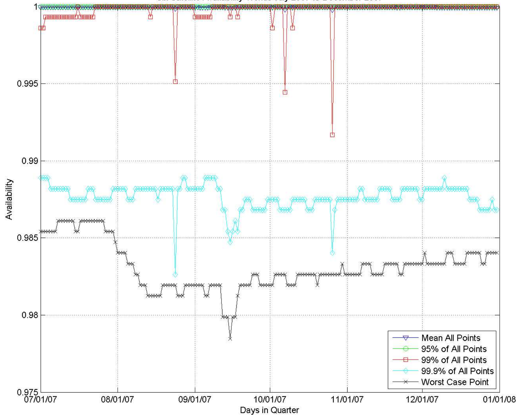
Six Satellite Availability Trends July 2007 to December 2007
