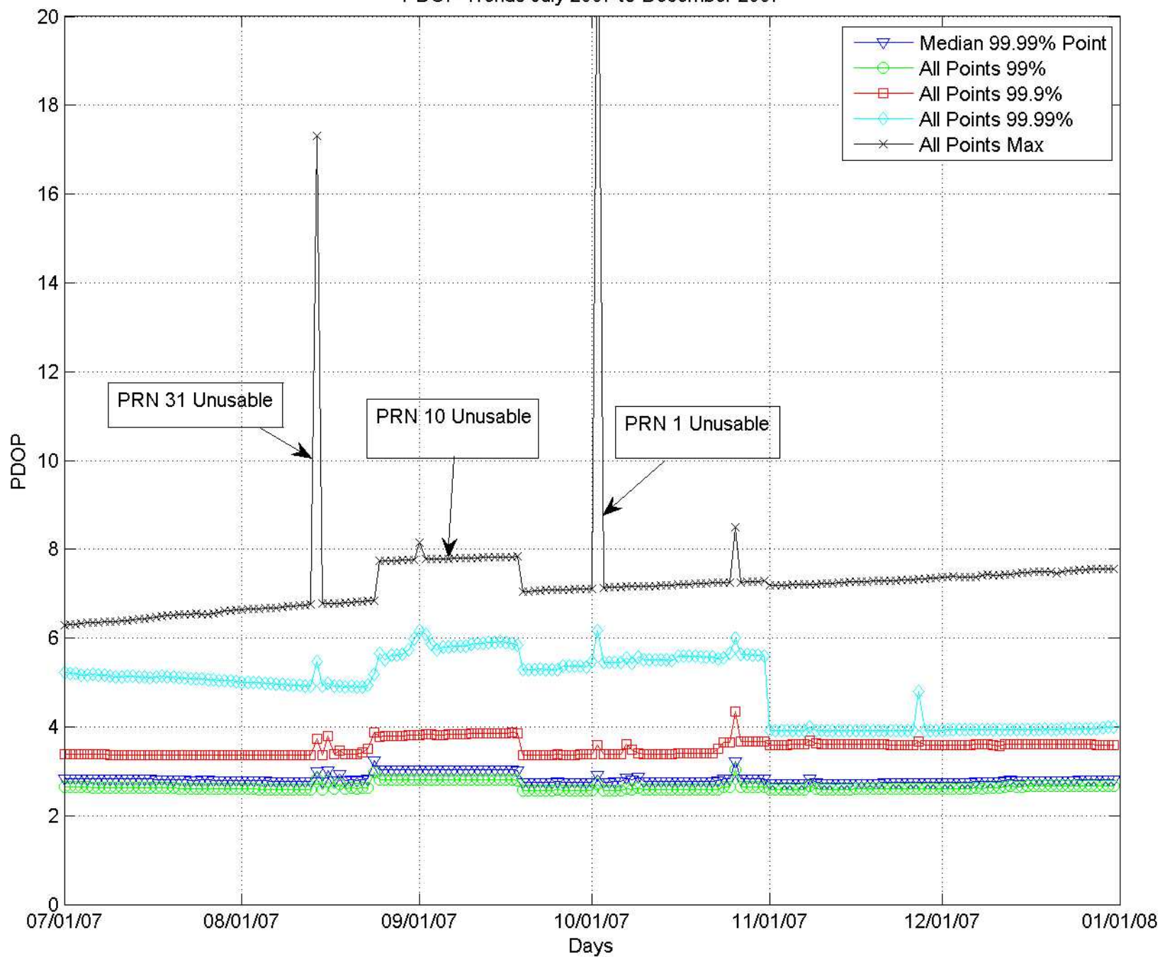
PDOP Trends July 2007 to December 2007
