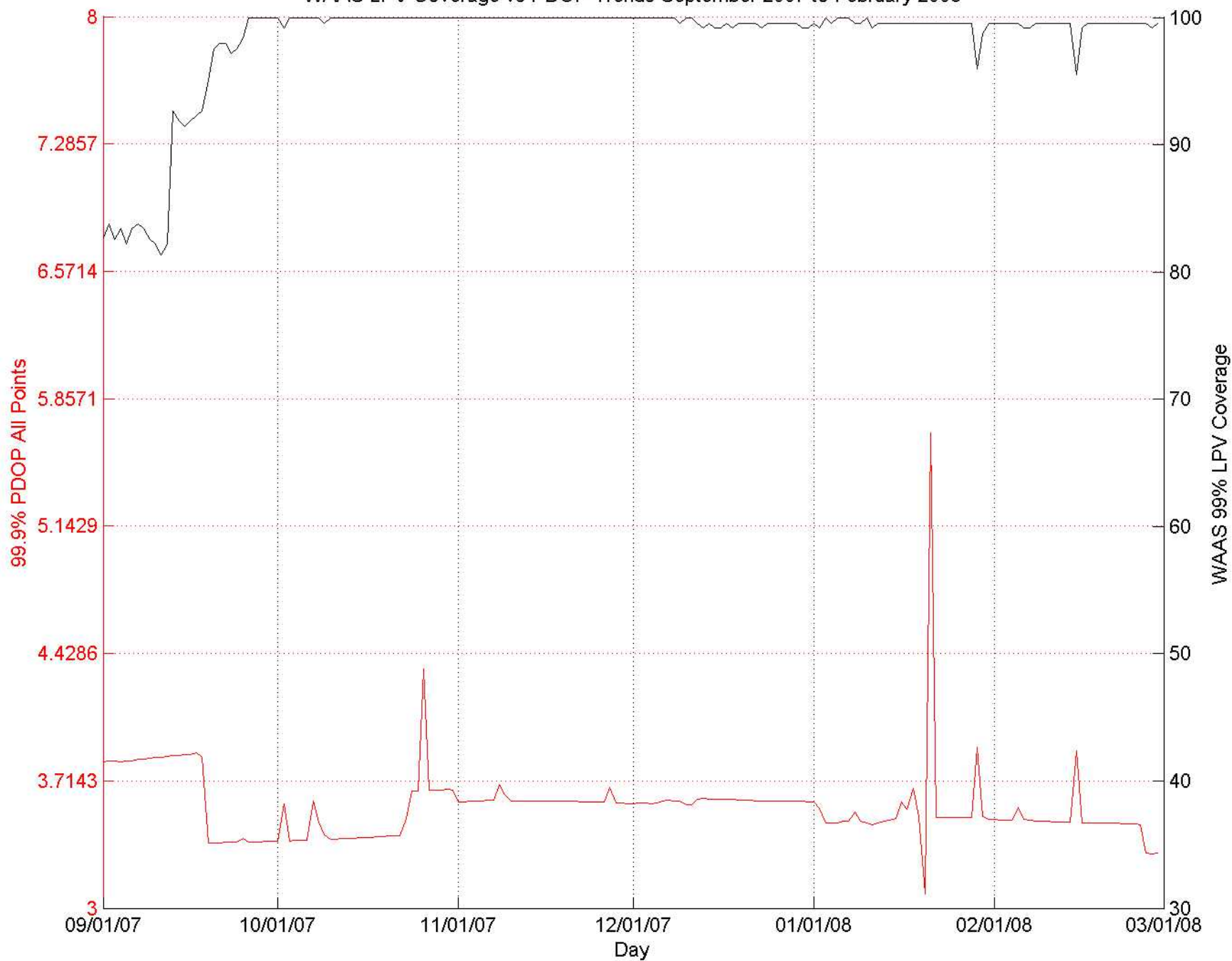
WAAS LPV Coverage vs PDOP Trends September 2007 to February 2008
