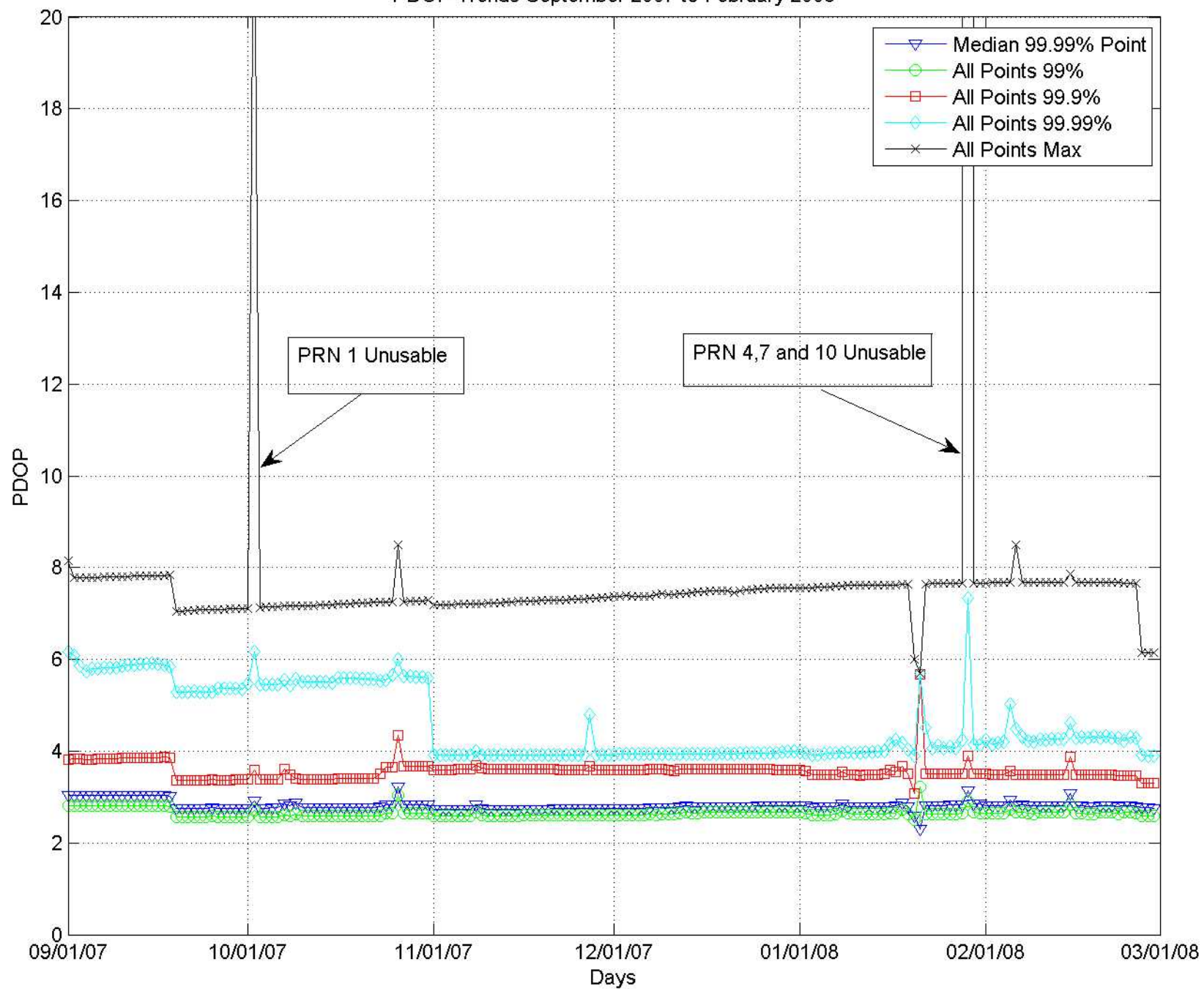
PDOP Trends September 2007 to February 2008
