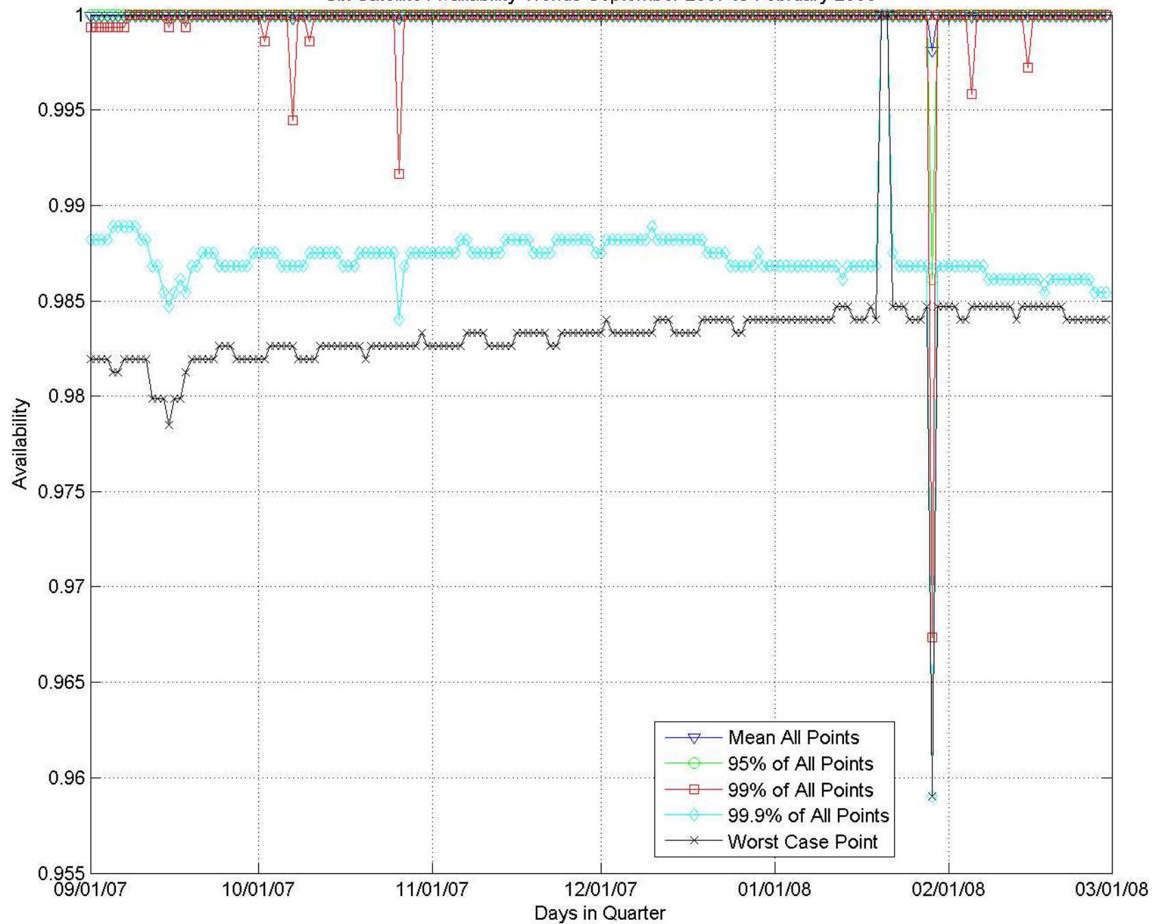
Six Satellite Availability Trends September 2007 to February 2008
