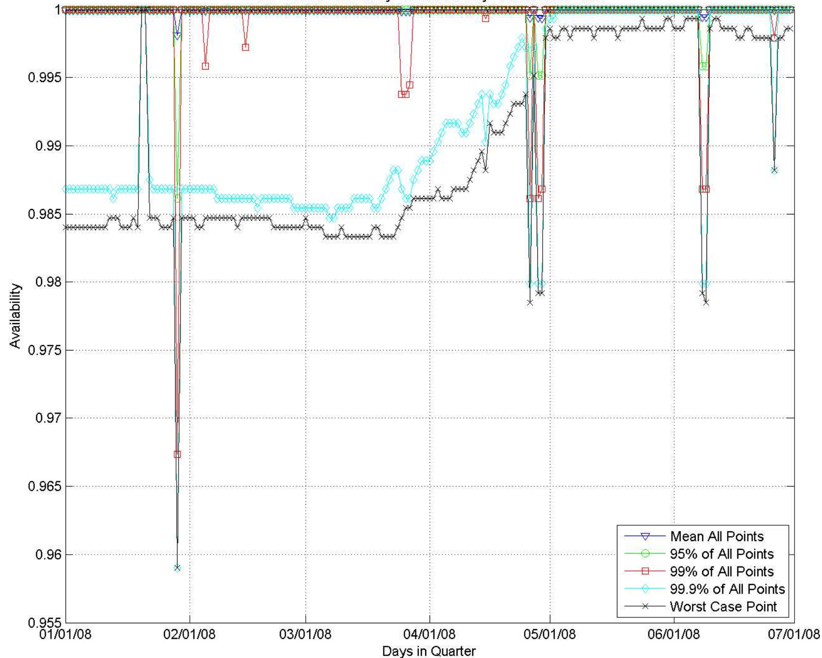
Six Satellite Availability Trends January 2008 to June 2008
