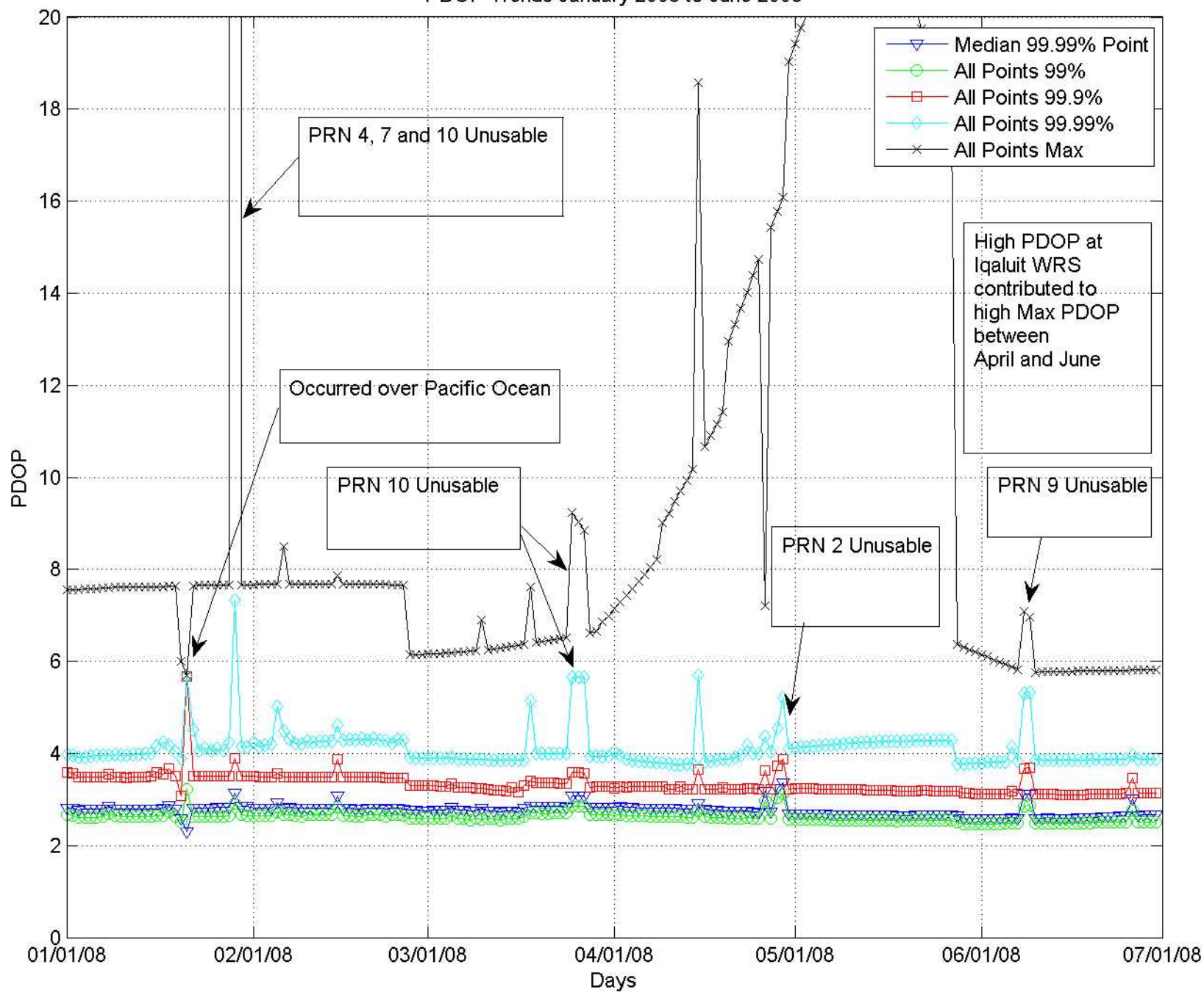
PDOP Trends January 2008 to June 2008
