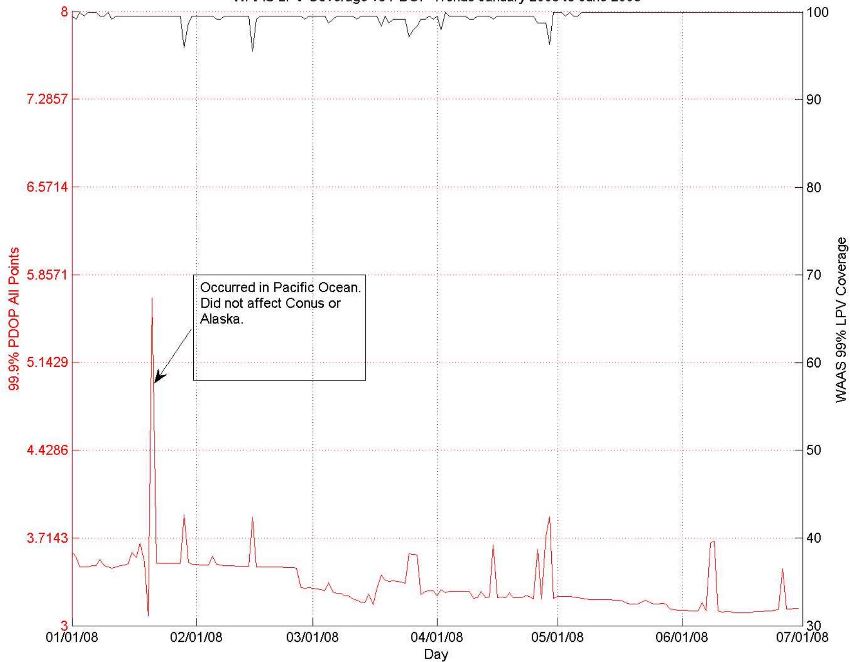
WAAS LPV Coverage vs PDOP Trends January 2008 to June 2008
