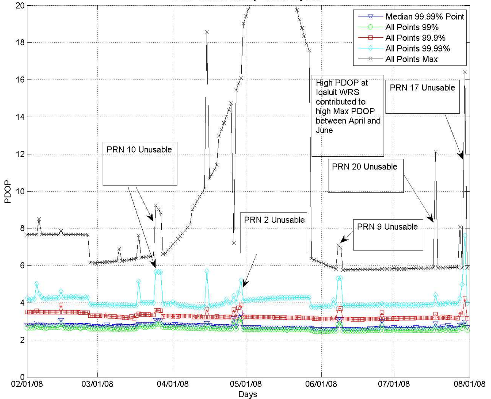
PDOP Trends February 2008 to July 2008
