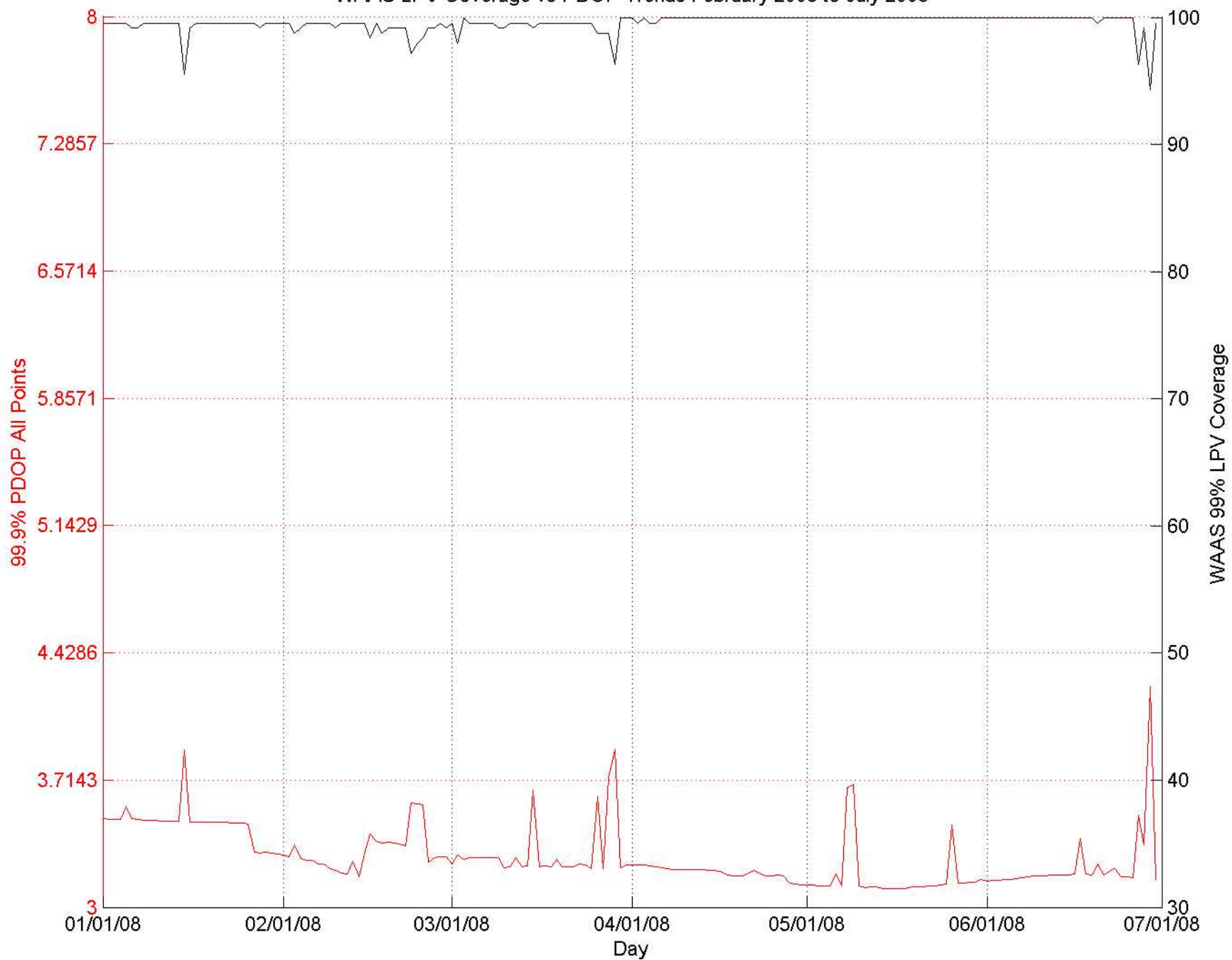
WAAS LPV Coverage vs PDOP Trends February 2008 to July 2008
