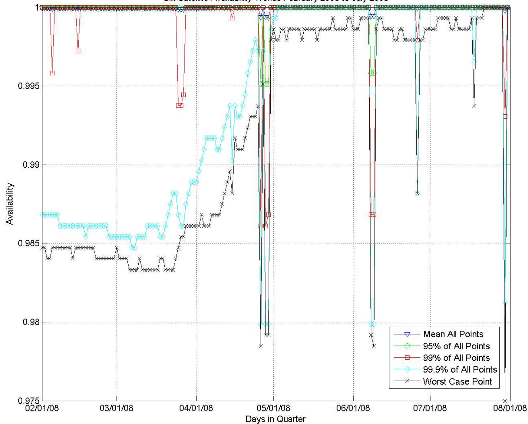
Six Satellite Availability Trends February 2008 to July 2008
