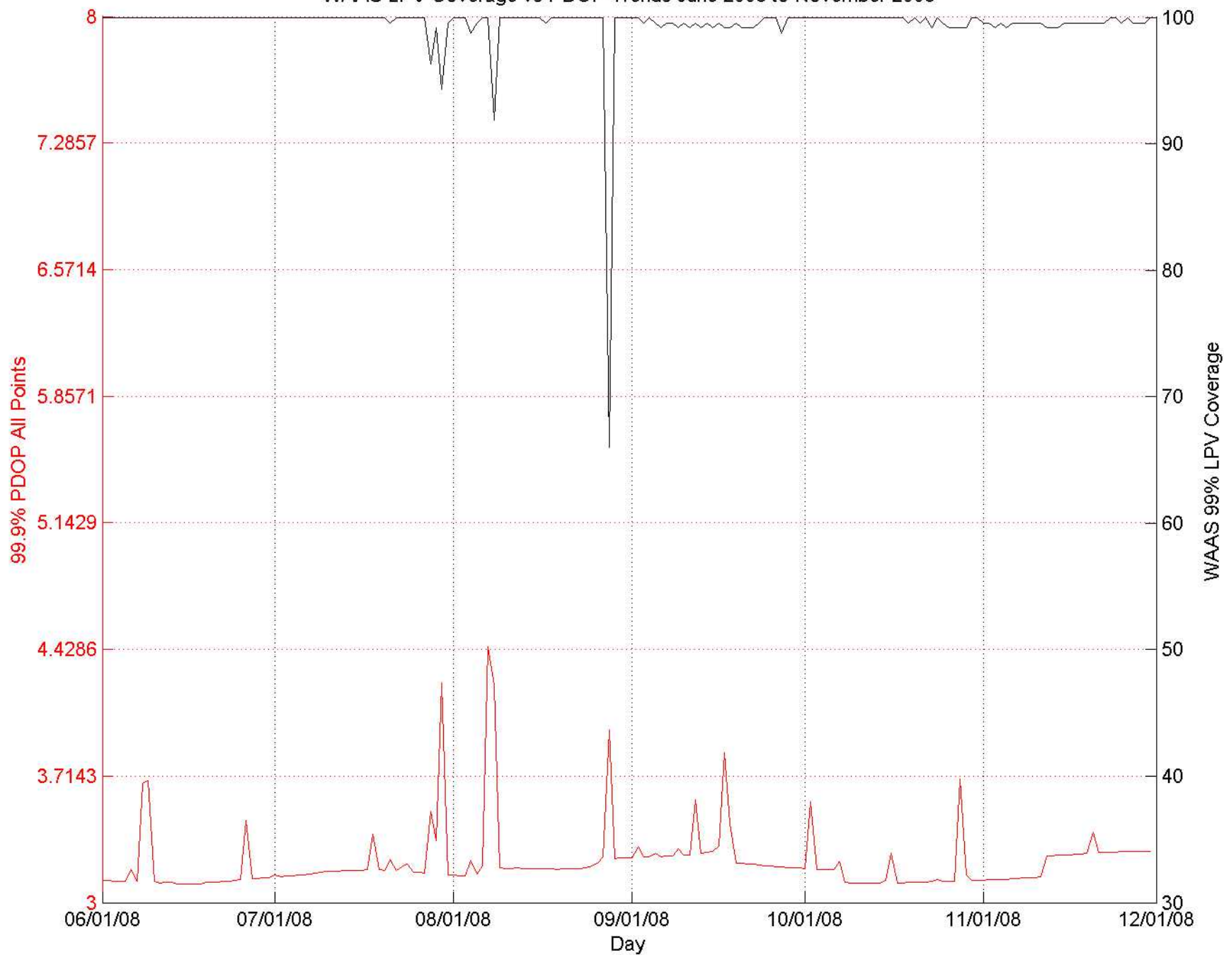
WAAS LPV Coverage vs PDOP Trends June 2008 to November 2008
