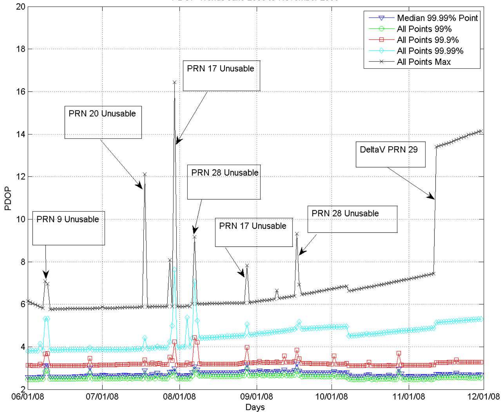
PDOP Trends June 2008 to November 2008
