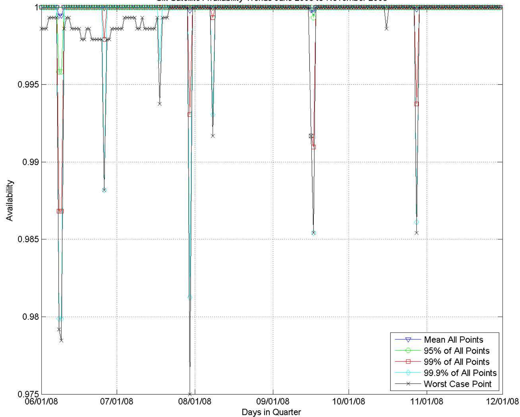
Six Satellite Availability Trends June 2008 to November 2008
