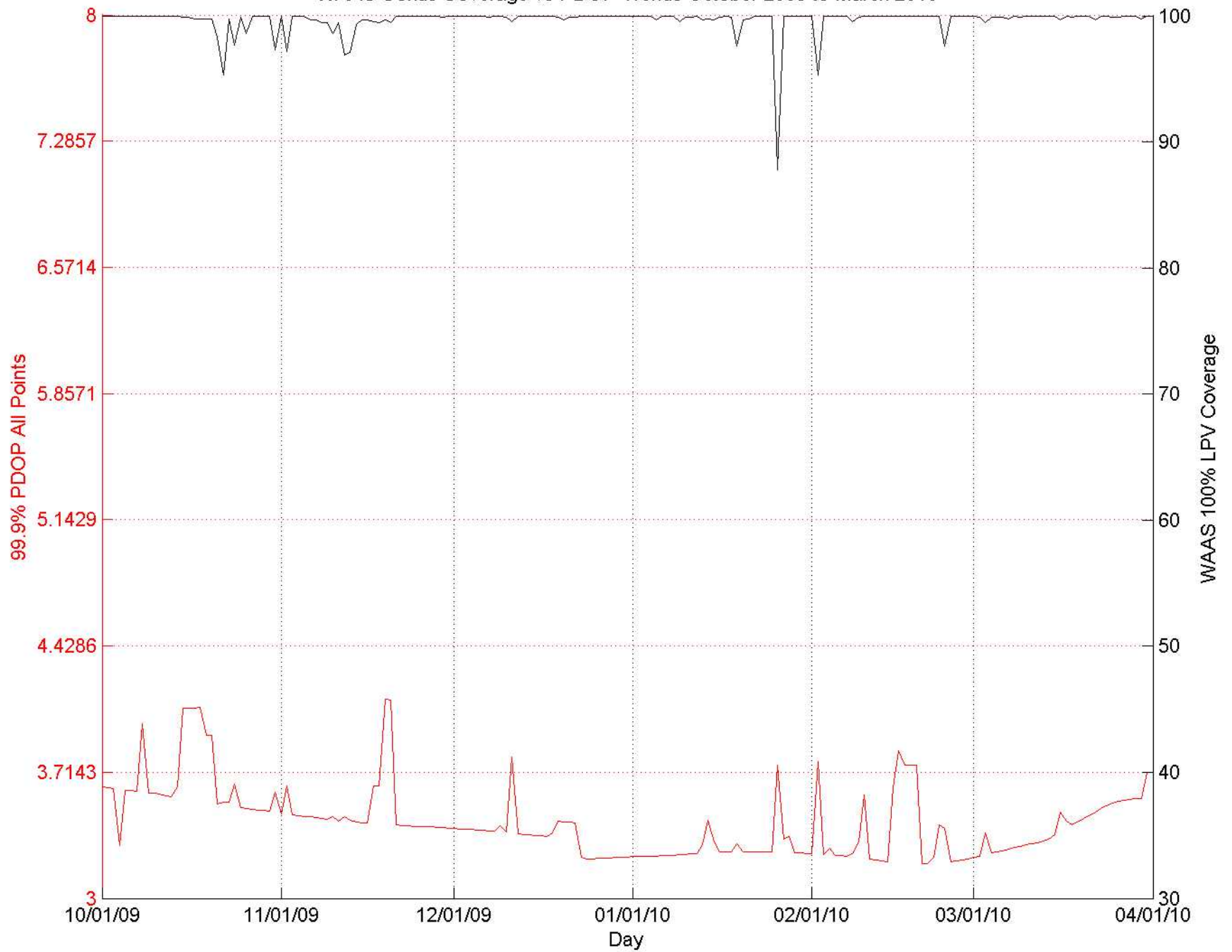
WAAS Conus Coverage vs PDOP Trends October 2009 to March 2010
