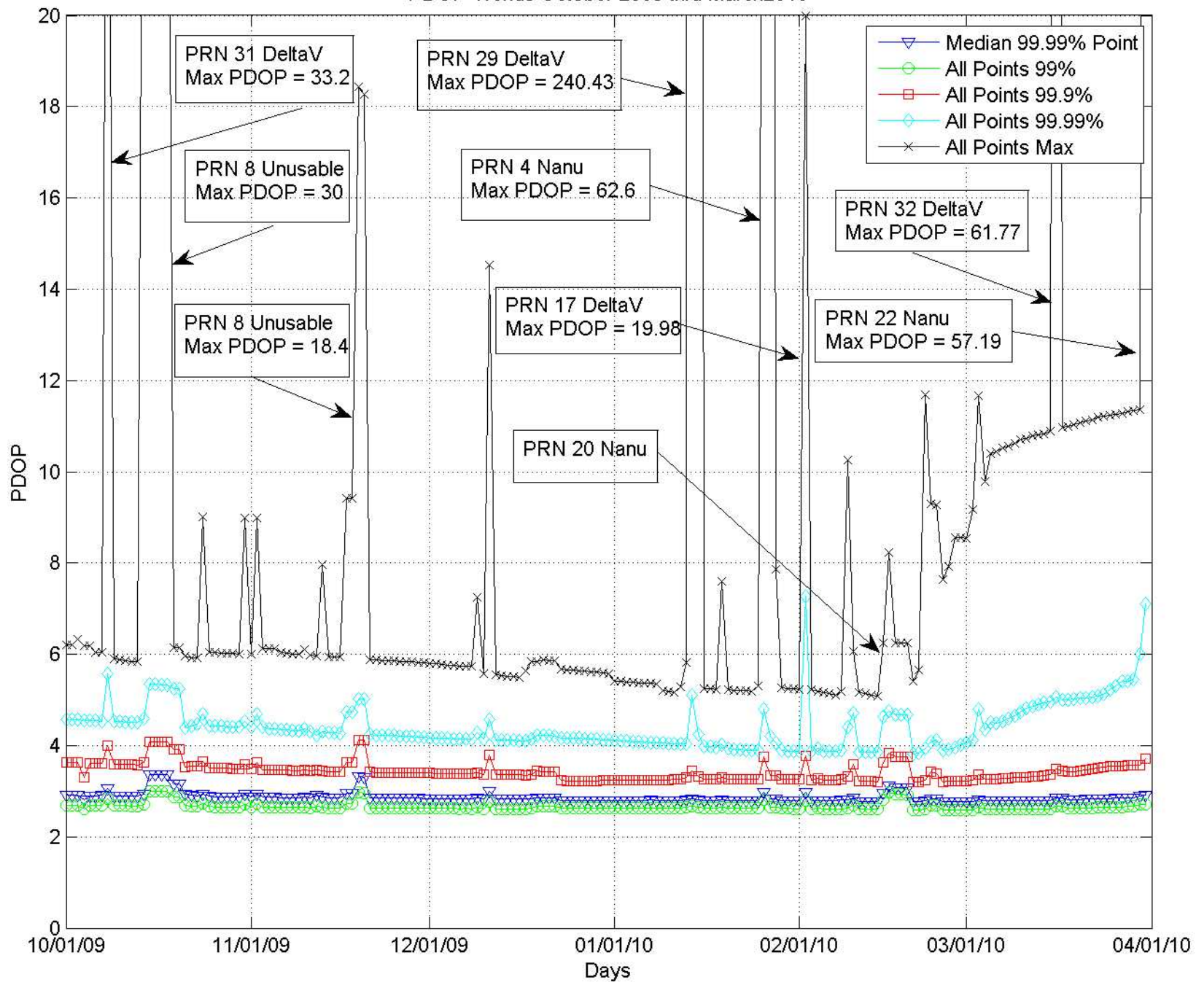
PDOP Trends October 2009 thru March2010
