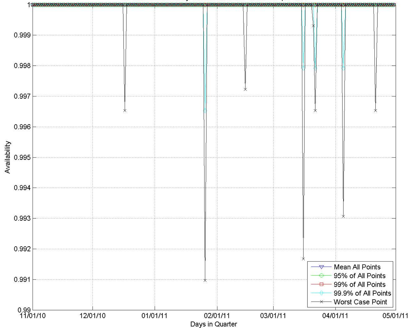
Six Satellite Availability Trends November 2010 thru April 2011
