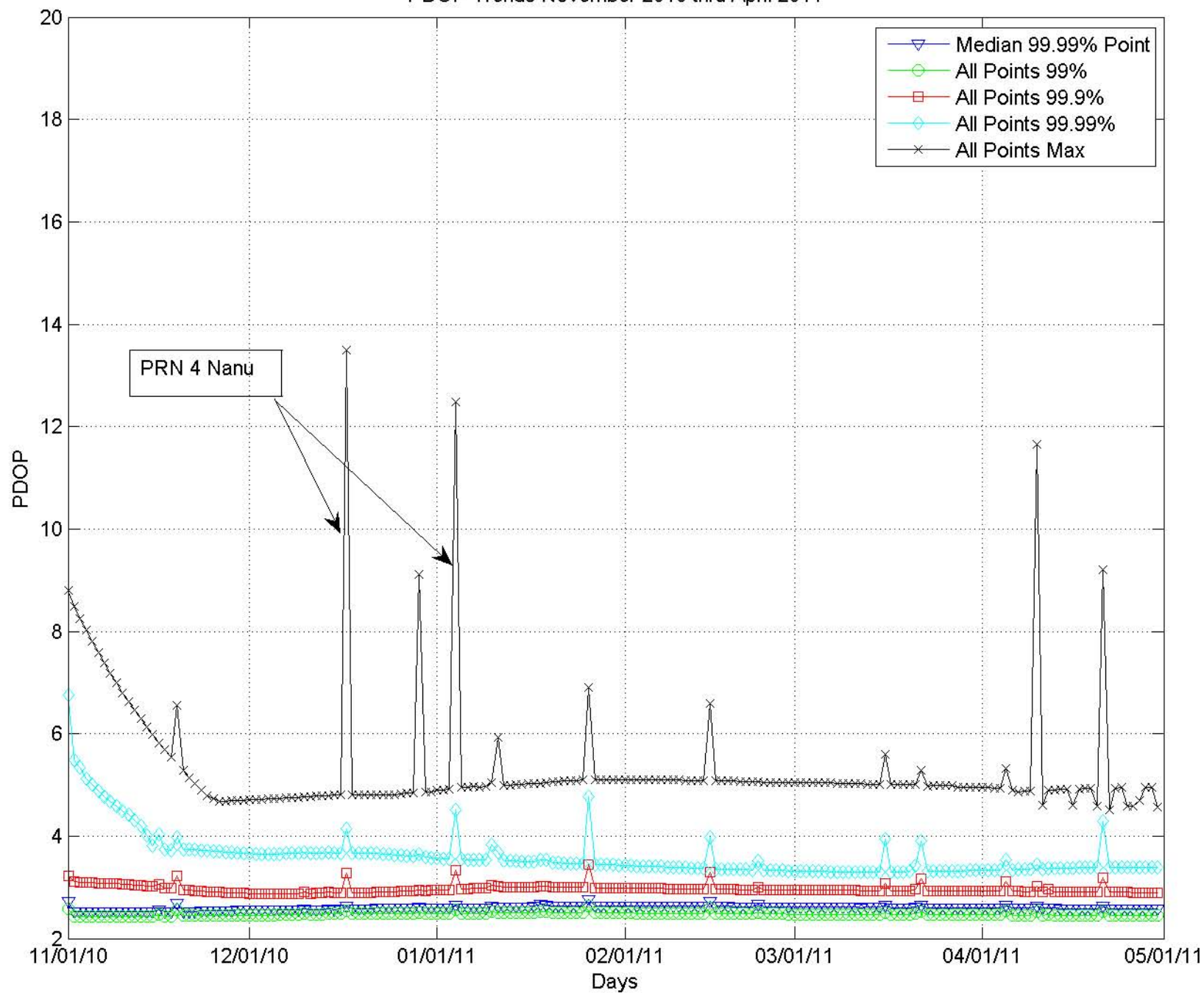
PDOP Trends November 2010 thru April 2011
