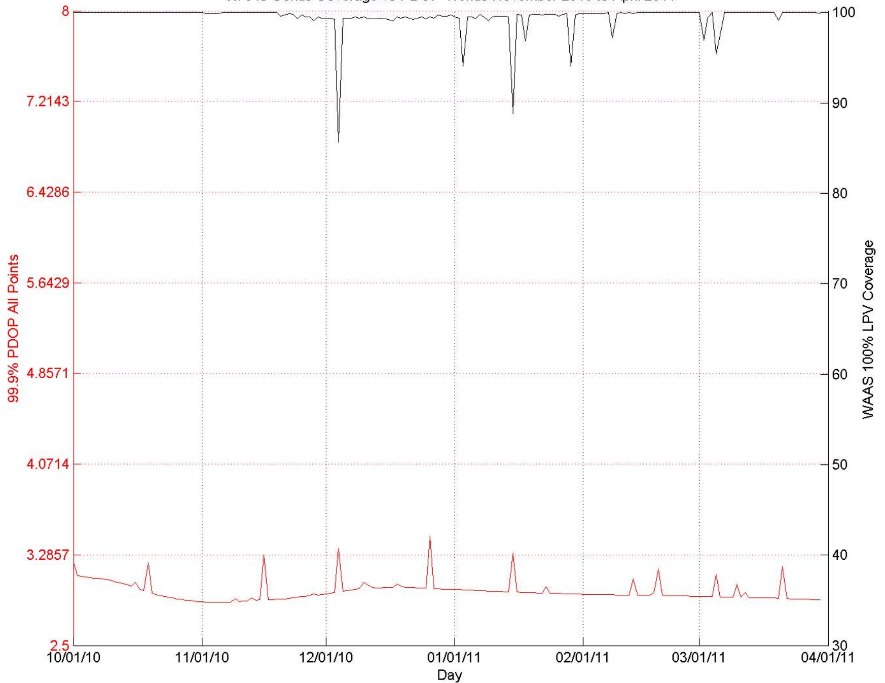
WAAS Conus Coverage vs PDOP Trends November 2010 to April 2011
