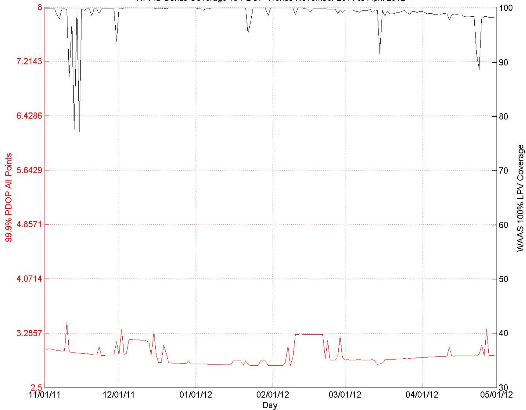
WAAS Conus Coverage vs PDOP Trends November 2011 to April 2012
