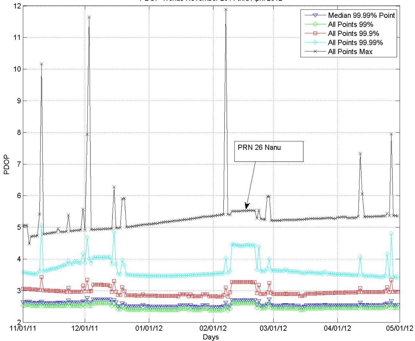
PDOP Trends November 2011 thru April 2012
