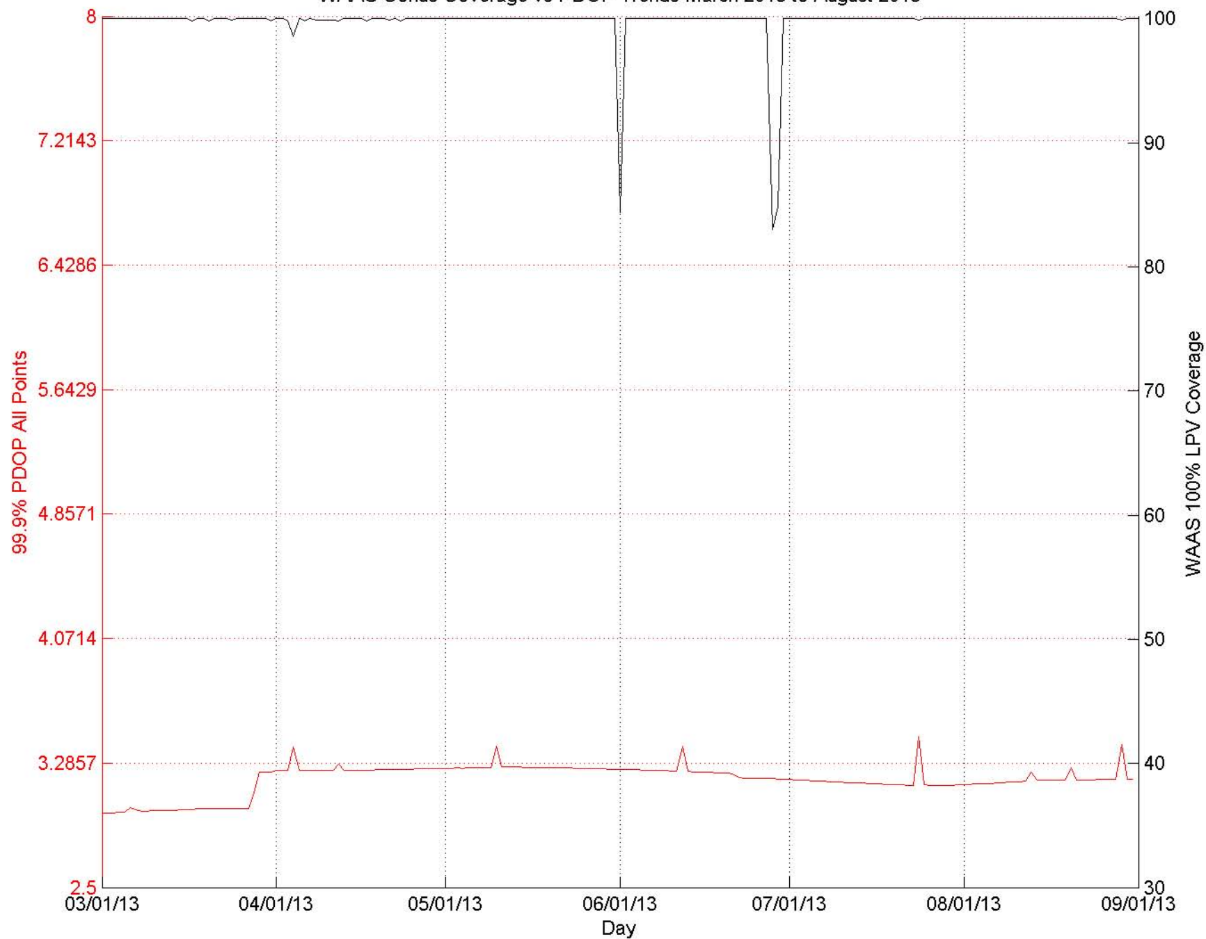
WAAS Conus Coverage vs PDOP Trends March 2013 to August 2013
