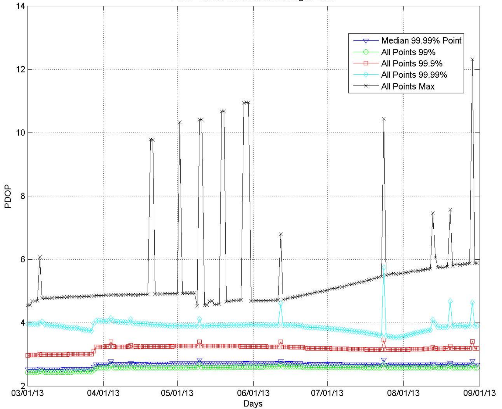
PDOP Trends March 2013 thru August 2013
