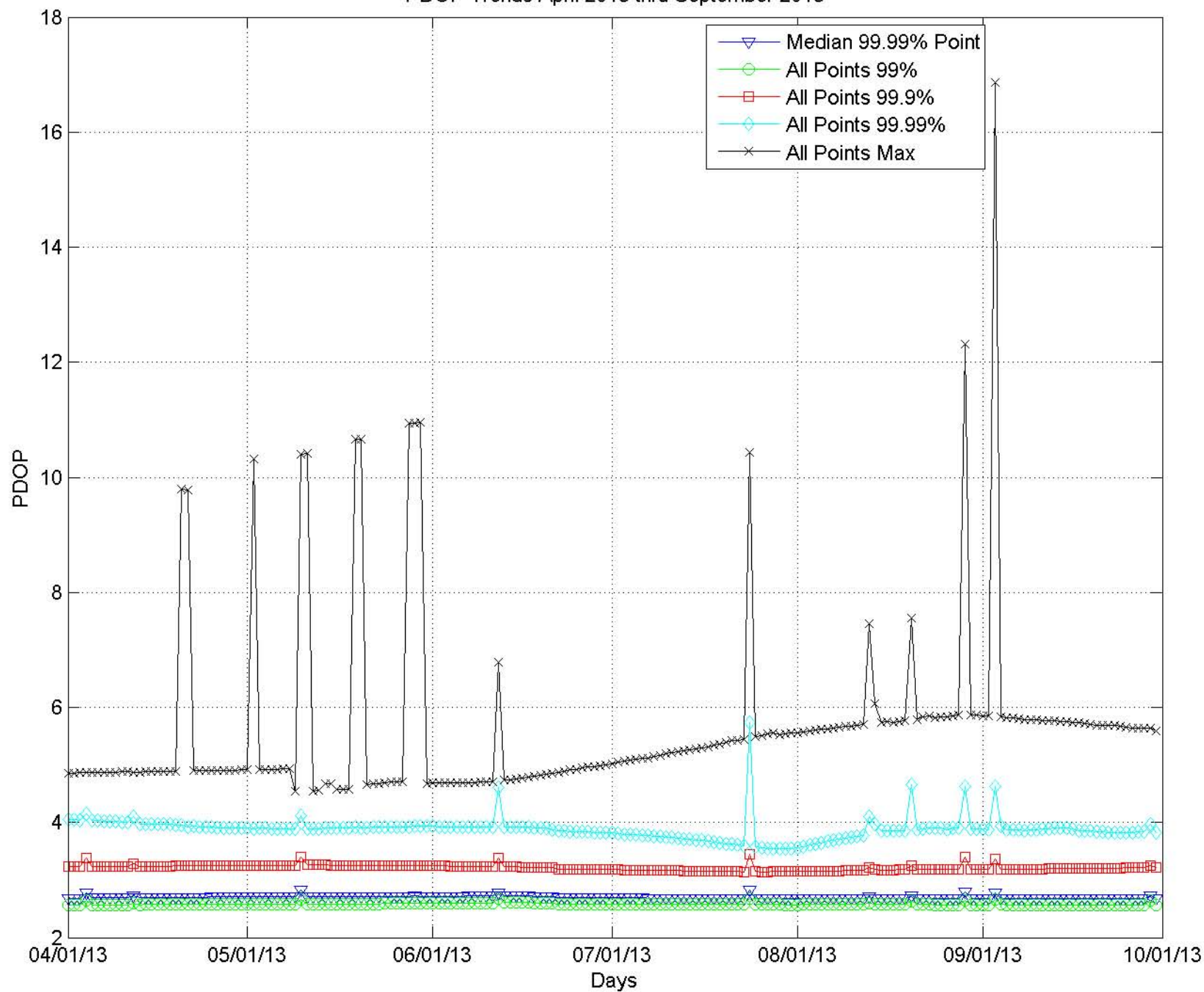
PDOP Trends April 2013 thru September 2013
