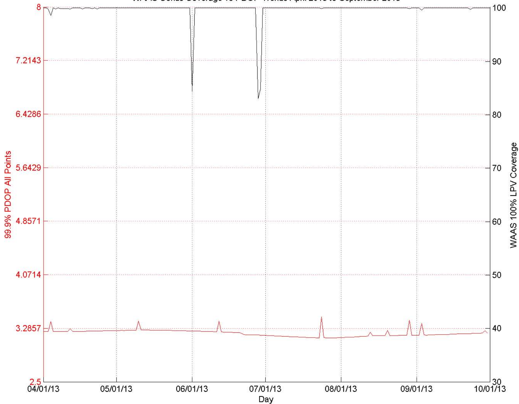
WAAS Conus Coverage vs PDOP Trends April 2013 to September 2013
