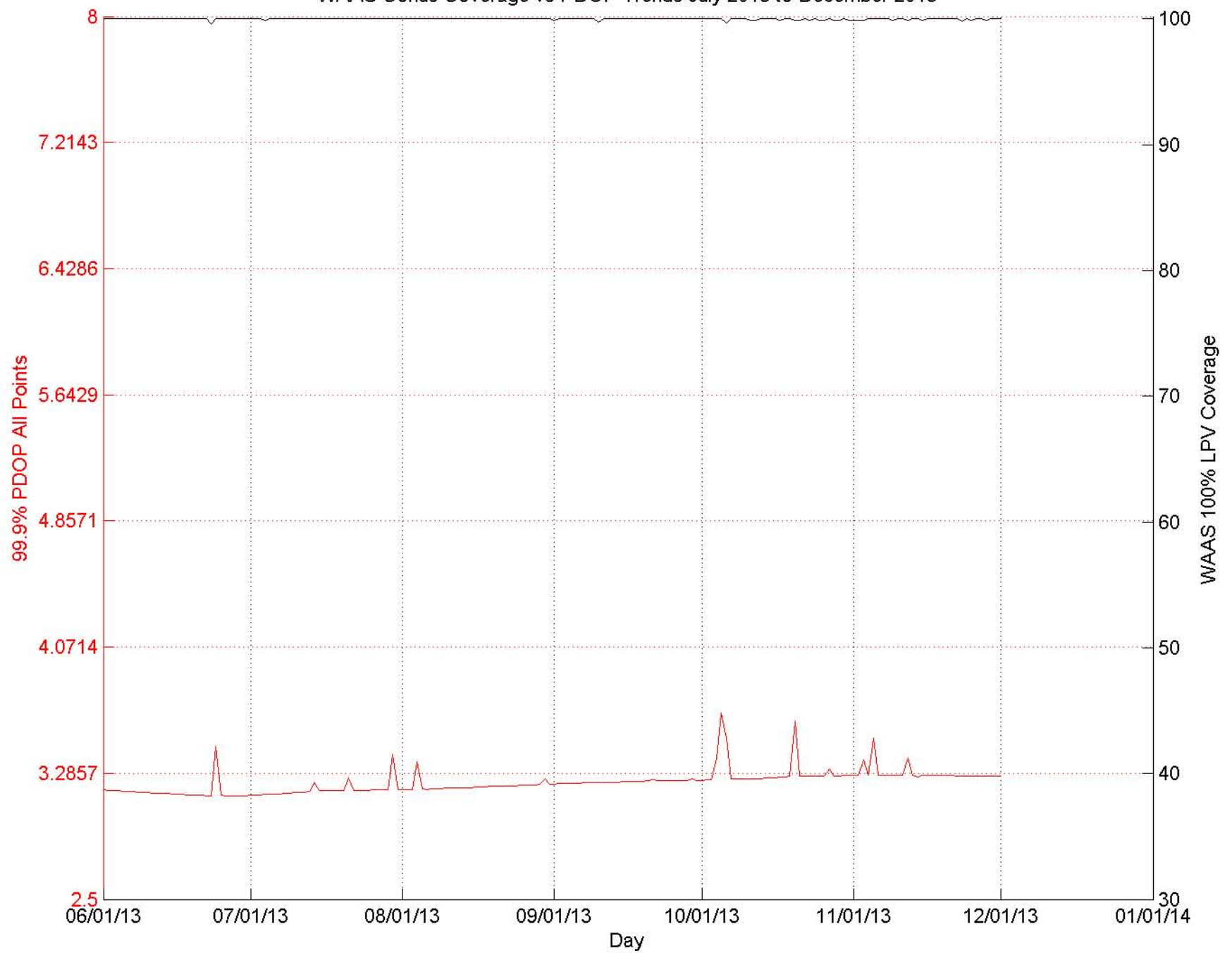
WAAS Conus Coverage vs PDOP Trends July 2013 to December 2013
