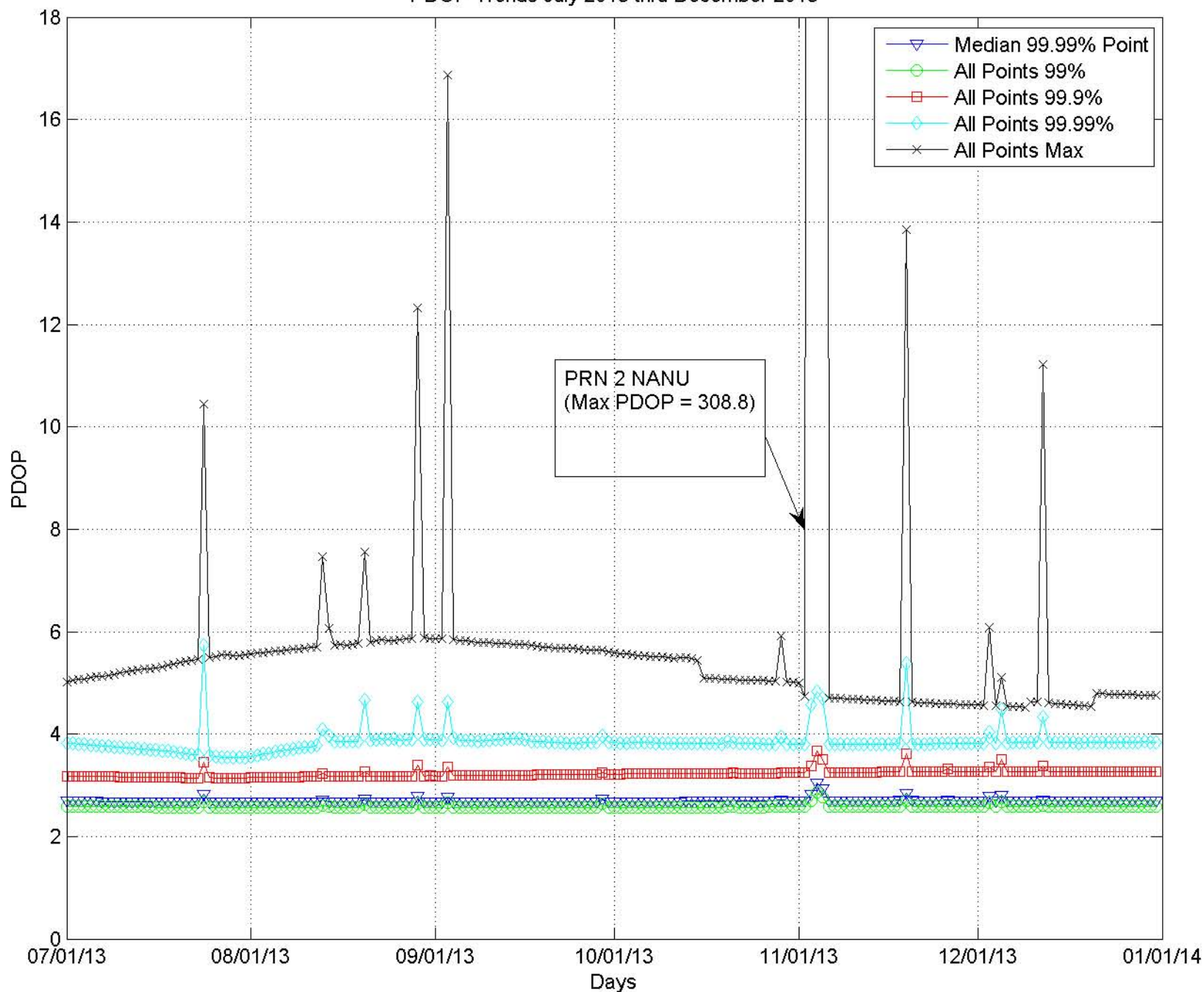
PDOP Trends July 2013 thru December 2013
