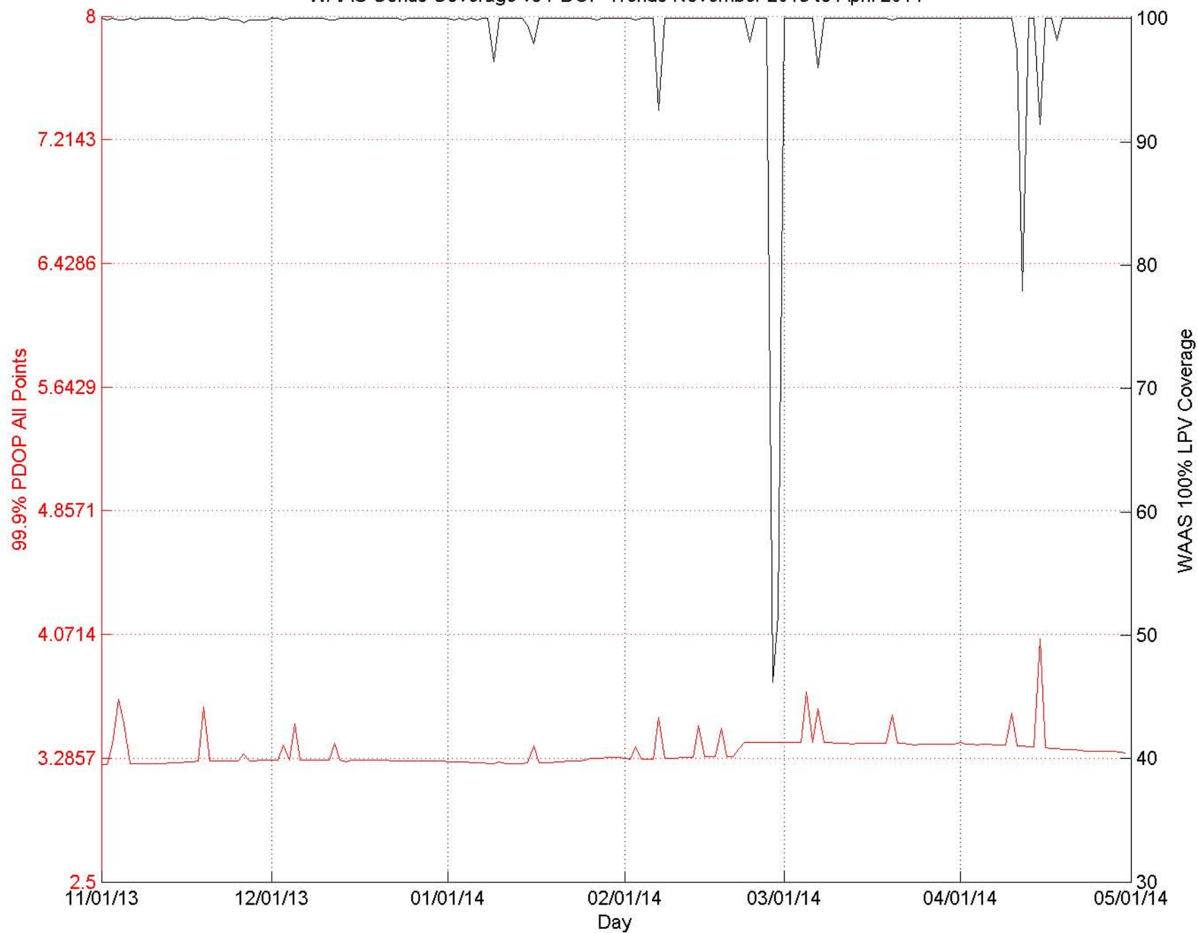
WAAS Conus Coverage vs PDOP Trends November 2013 to April 2014
