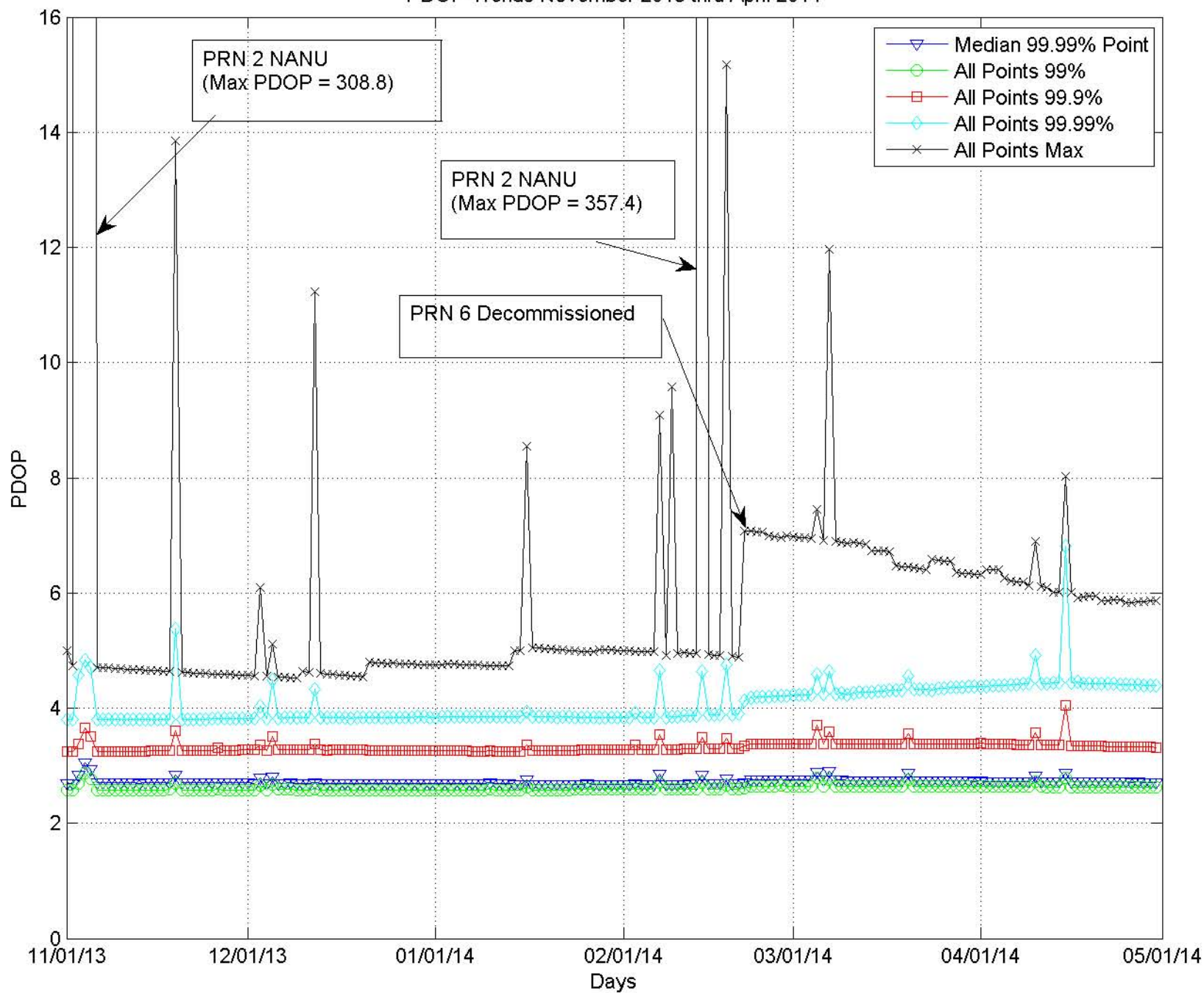
PDOP Trends November 2013 thru April 2014
