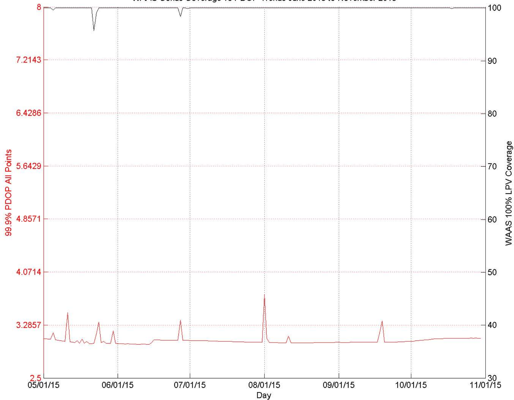
WAAS Conus Coverage vs PDOP Trends June 2015 to November 2015
