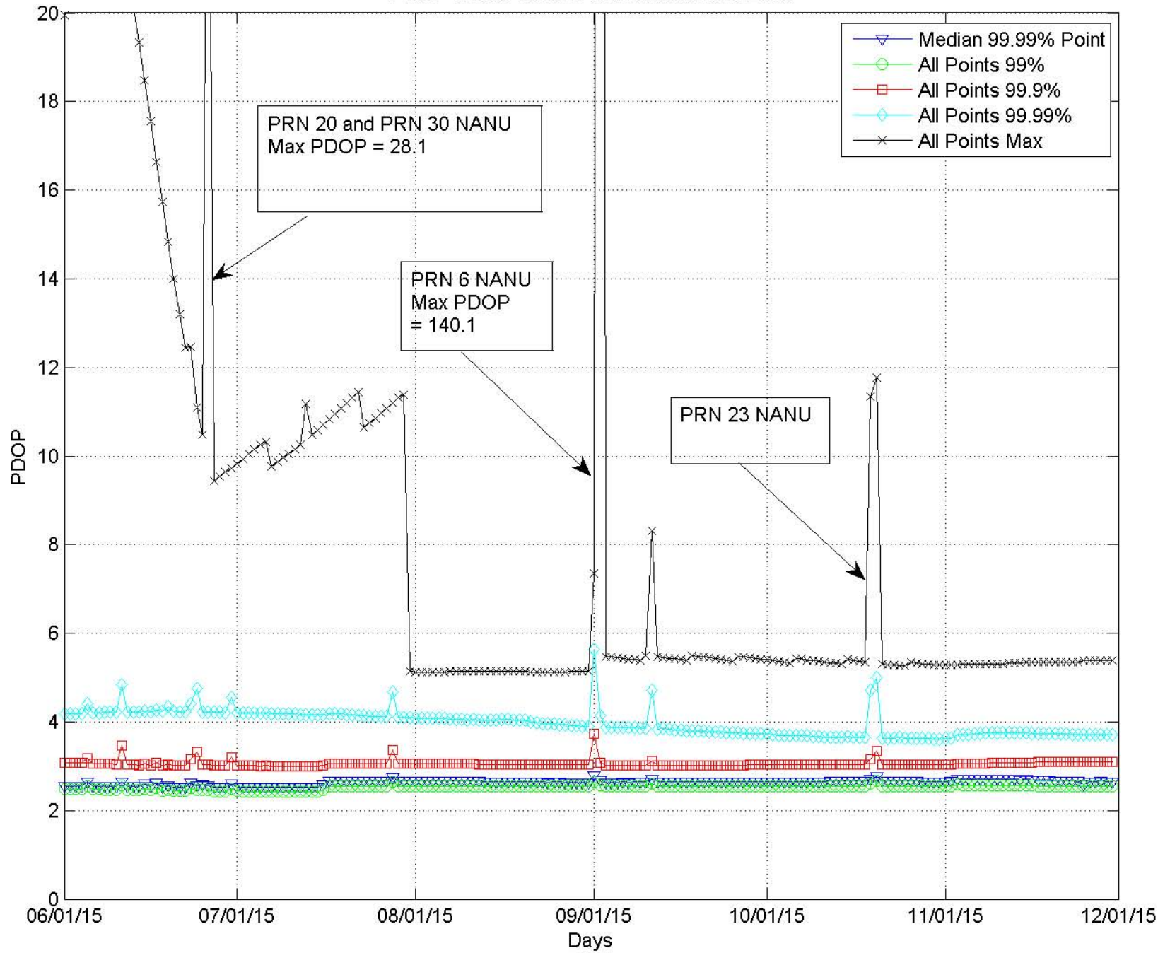
PDOP Trends June 2015 thru November 2015
