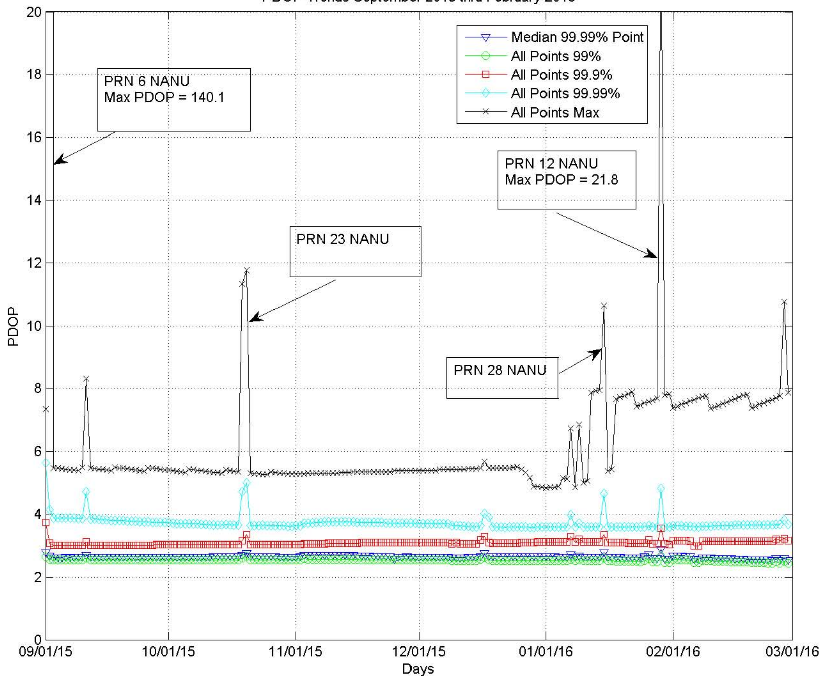
PDOP Trends September 2015 thru February 2016
