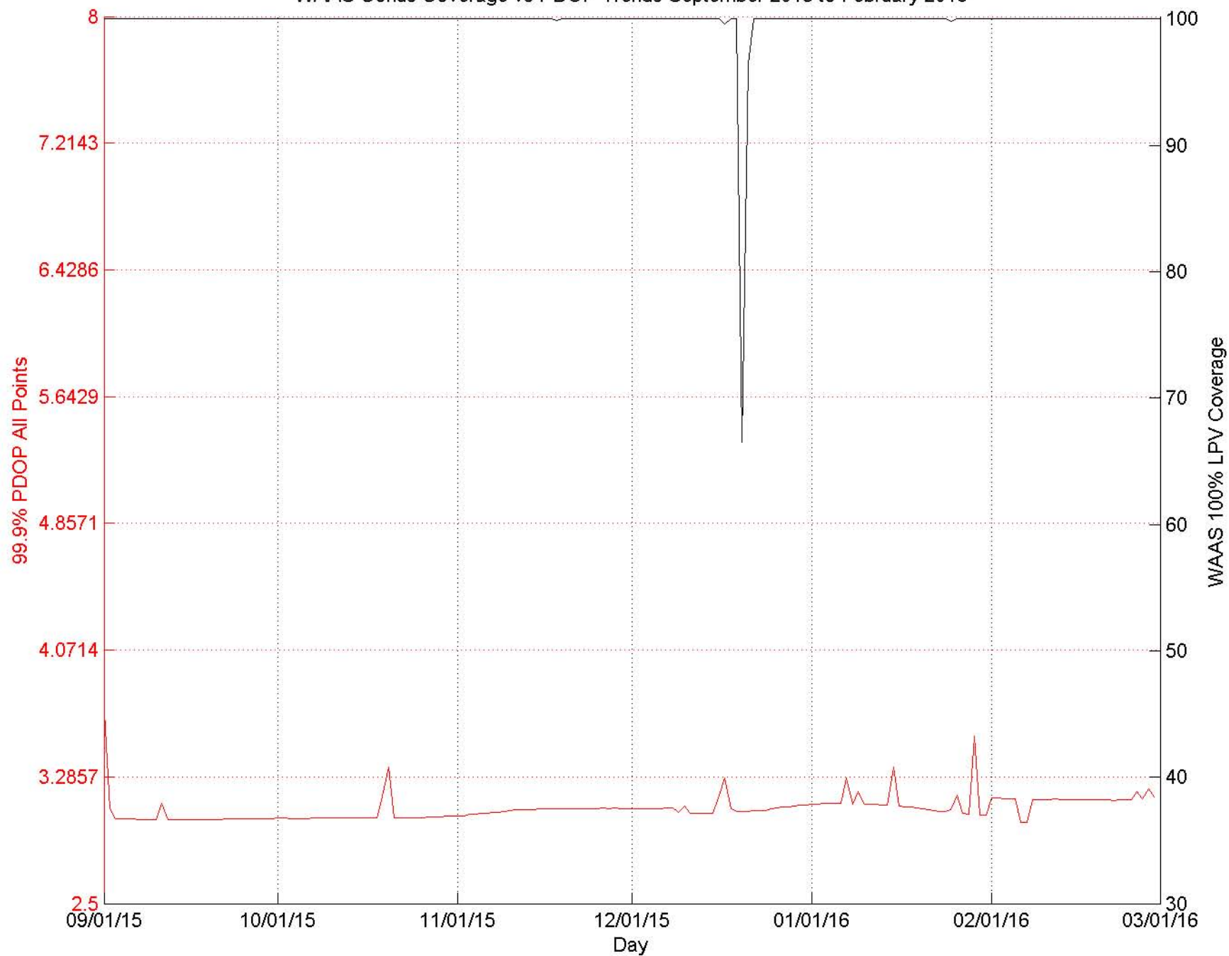
WAAS Conus Coverage vs PDOP Trends September 2015 to February 2016
