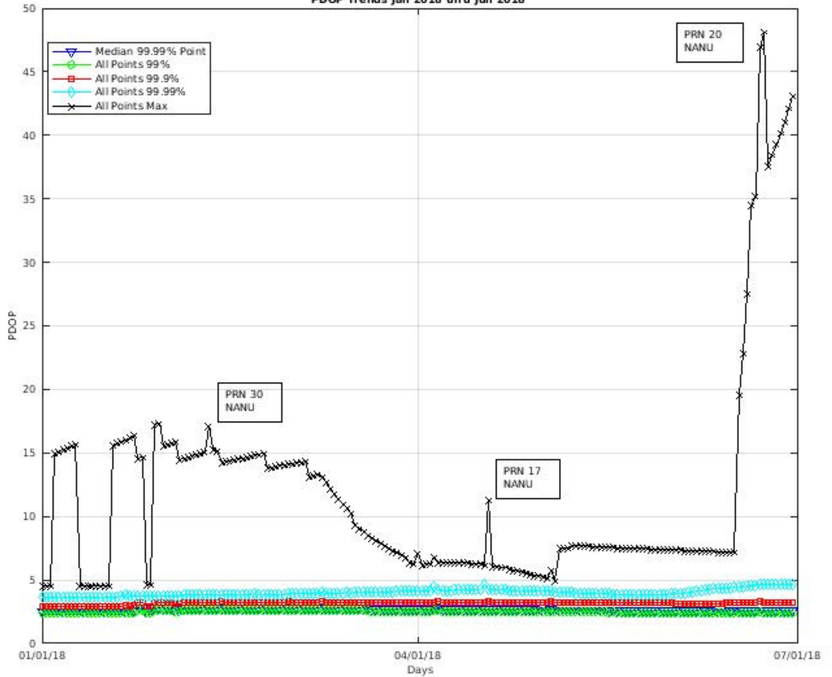
PDOP Trends Jan 2018 thru Jun 2018
