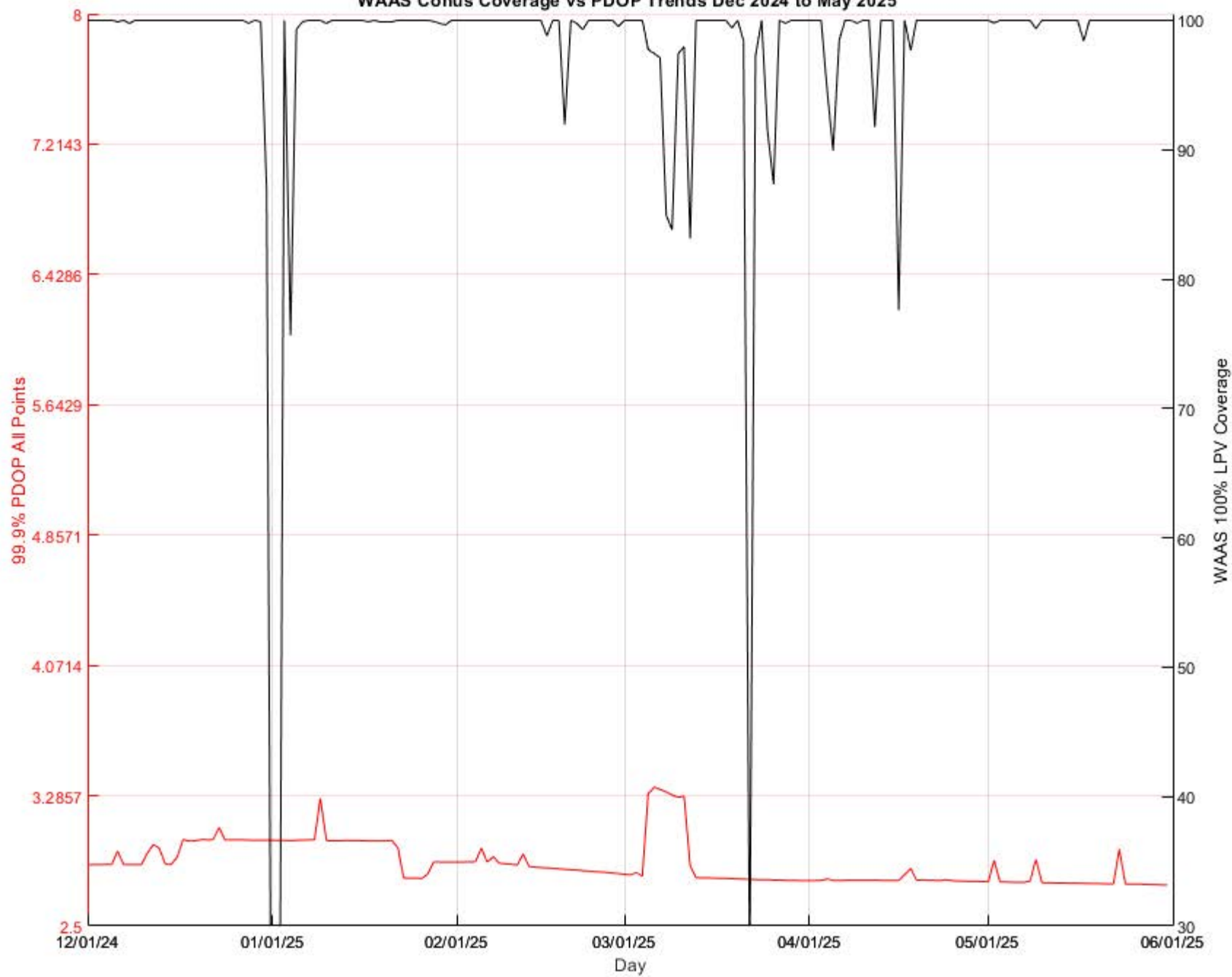
WAAS Conus Coverage vs PDOP Trends Dec 2024 to May 2025
