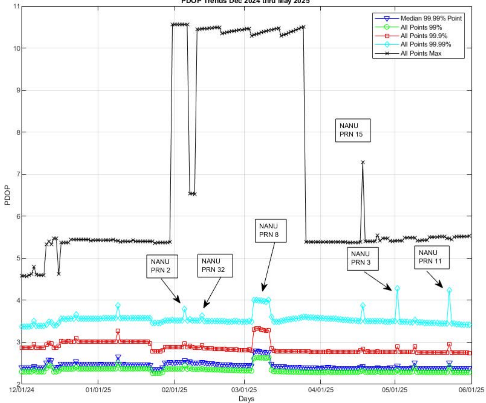
PDOP Trends Dec 2024 thru May 2025
